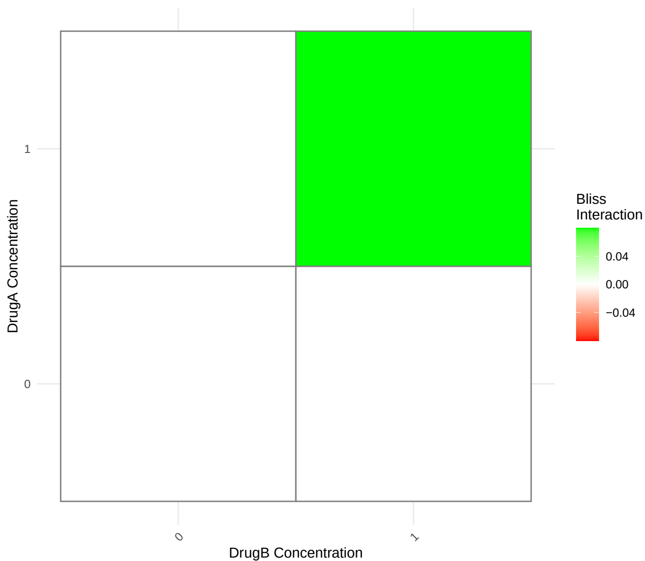
Bliss Interaction Surface: DrugA + DrugB
