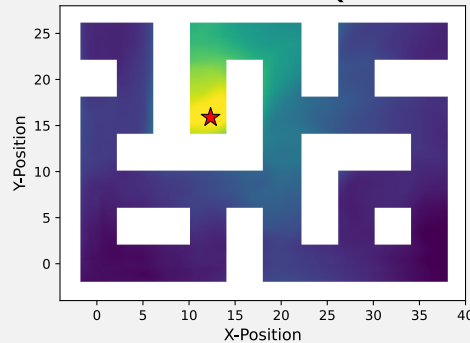
GCIVL + IQE
