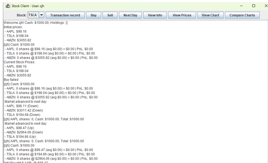
Figure 1: stock client
