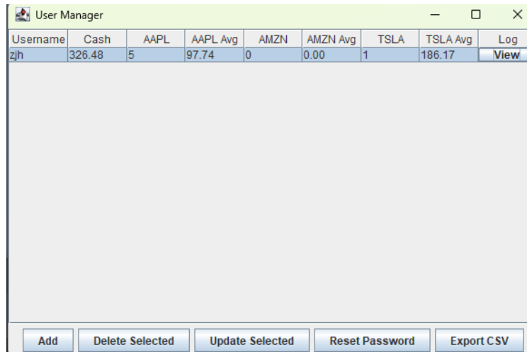
Figure 7: user manager
