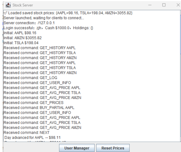
Figure 6: stock server
