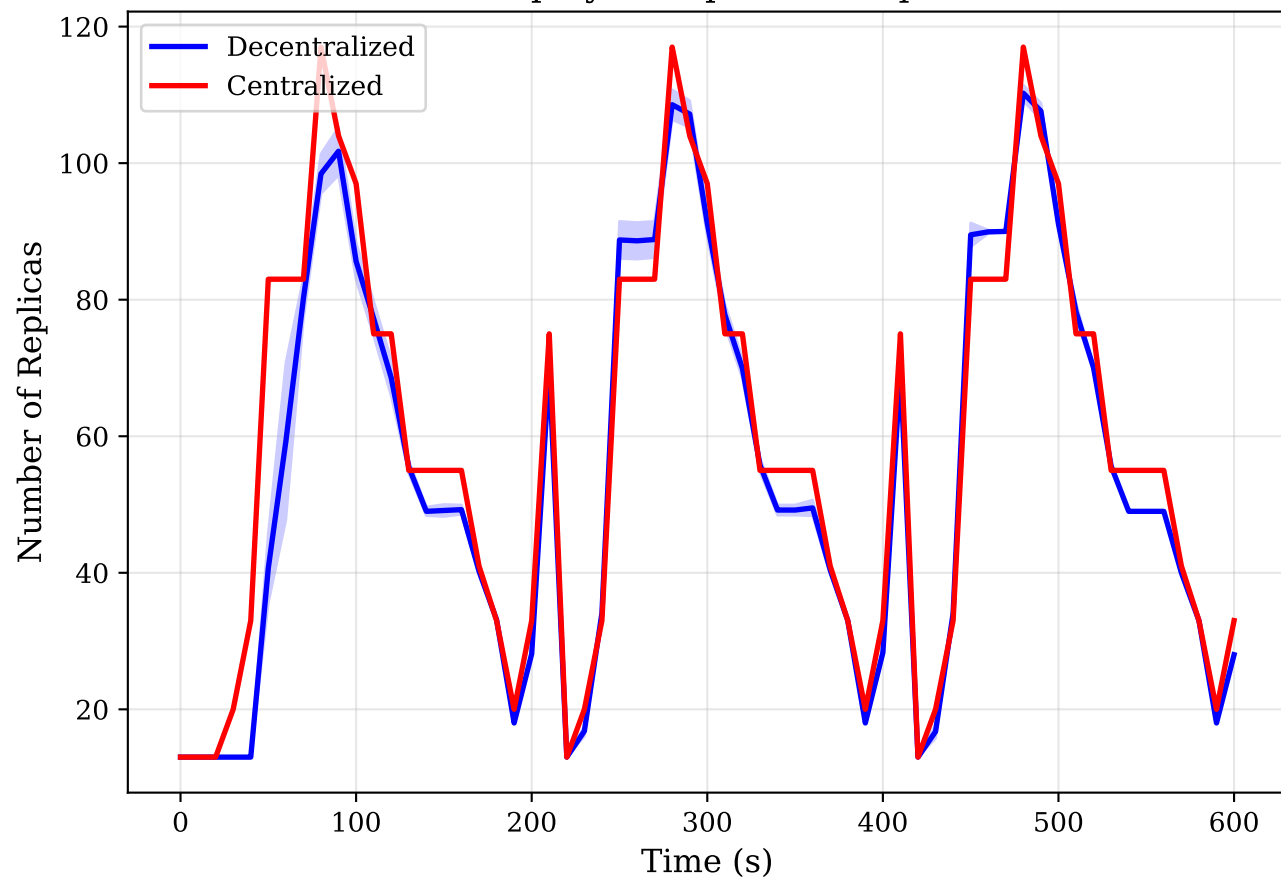
Total Deployed Replicas Comparison
