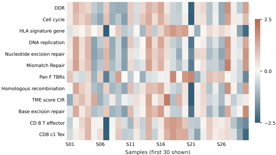
Variation in signature-specific PC1 scores
