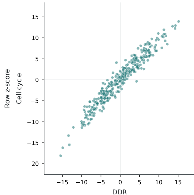
Two signature axes · all 348 samples
