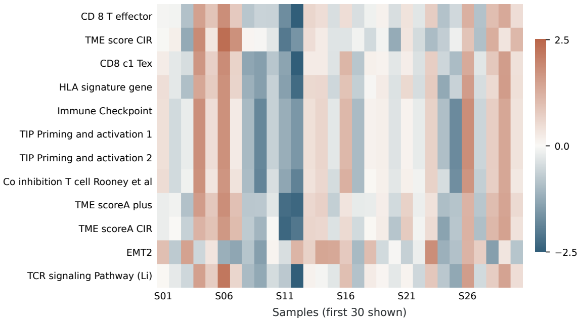
Relative enrichment across samples
