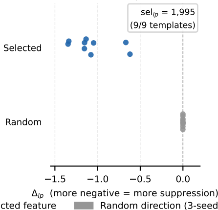
(b) Rare positive control: Llama L16 / name
