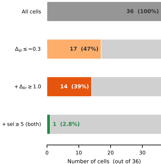
(a) Single-metric success collapses under multi-metric evaluation
