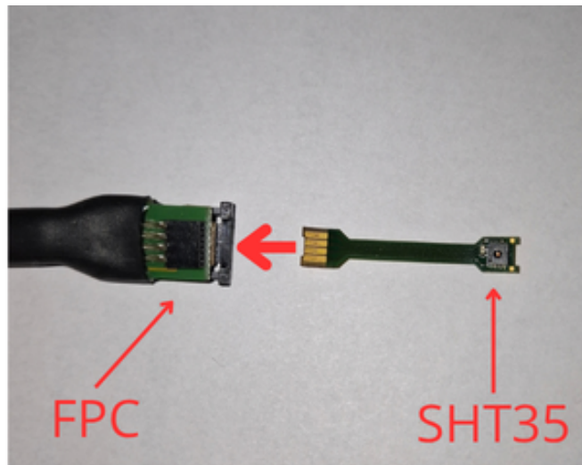
Figure 3: SHT35 sensor
