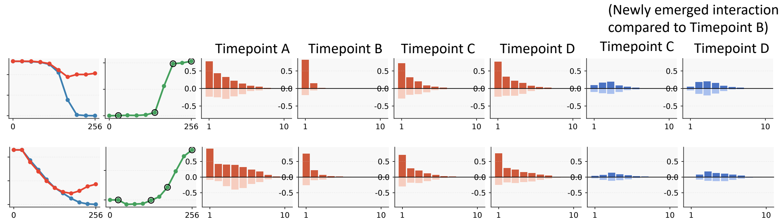
Caption: Overfitting-phase analysis. From left to right, we present the training dynamics, the raw interaction distributions at time points A, B, C, and D, and the newly emerged interaction distributions defined by the differences between C and B, and D and B. The newly emerged interactions exhibit a clear spindle-shaped pattern, supporting the view that overfitting primarily introduces noise-like interactions.
