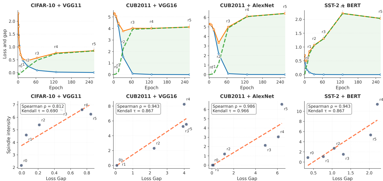
Caption. (Top) Train loss, test loss, and their gap (test loss – train loss) across epochs. (Bottom) Scatter plots of magnitude of spindled-shaped distribution and the loss gap across different timepoints, with Spearman's \rho and Kendall's \tau . High positive correlations indicate that a larger loss gap corresponds to a more pronounced spindle-shaped distribution, linking the spindle-shaped distribution of non-generalizable interaction to a the standard generalization metric, e.g. , loss gap.
