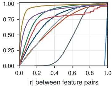
cumulative fraction
