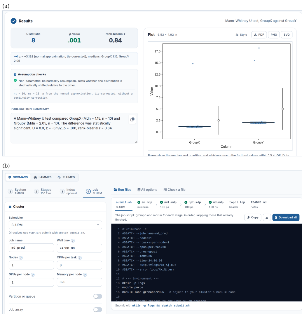
Figure 3: Listings 4 and 5 in the browser: (a) the statistics calculator comparing two groups, with the test the assumption checks pointed to, its effect size, a publication summary and the plot; (b) the MD workflow generator’s GROMACS job step and the submission script it writes.
