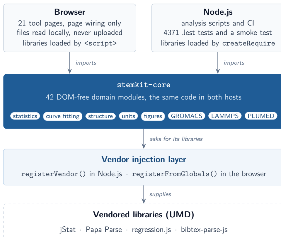
Figure 1: Architecture of STEMKit. Both hosts execute the identical core modules; the only environment-specific code is the registration call that supplies the vendored libraries.
