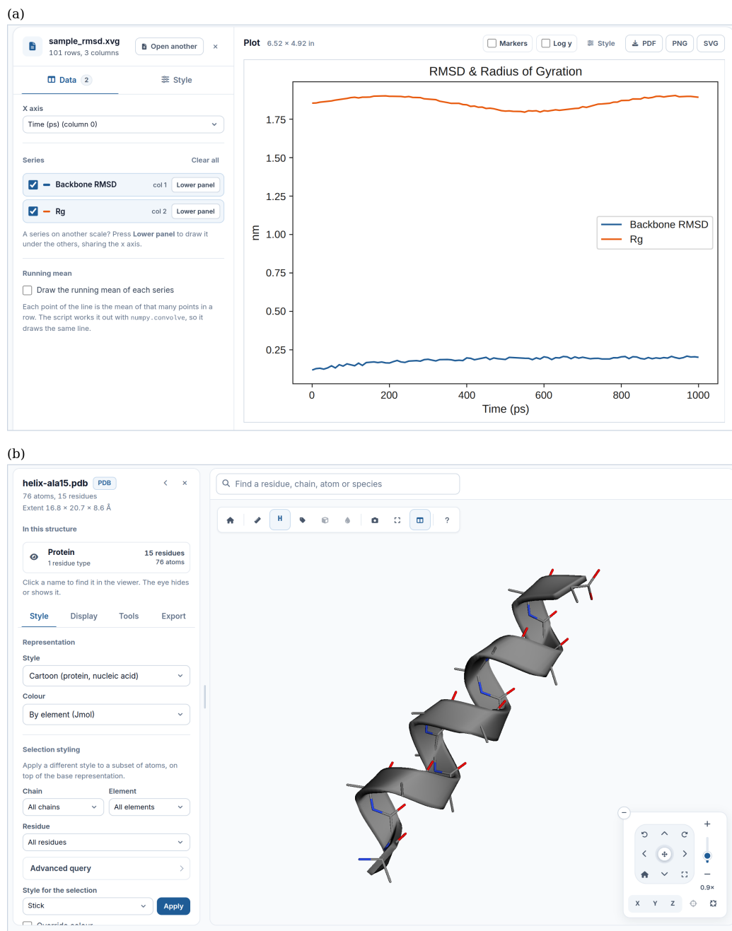
Figure 2: Listings 2 and 3 in the browser, with the tool pages' own samples: (a) the XVG visualiser plotting an RMSD and radius-of-gyration series; (b) the structure inspector with an \alpha -helical peptide.
