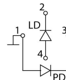
PINOUT #12
