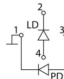
PINOUT #9
