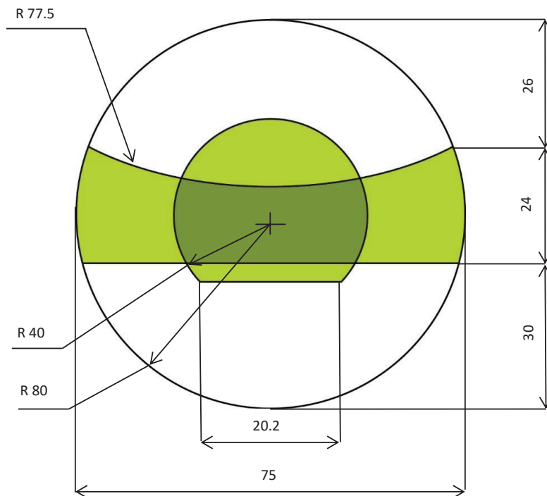
Figure 3 : Dimensions of the MEP label
