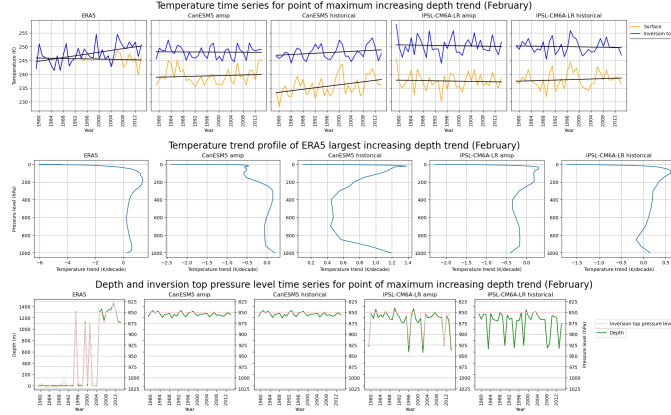
Figure 8: Inversion top and surface time series, trend profile, and depth and inversion top pressure level time series for the point of greatest increasing depth trend (75.75°N, 110.5°W in February)
