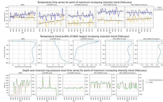
Figure 7: Inversion top and surface time series, trend profile, and depth and inversion top pressure level time series for the point of greatest increasing intensity trend (83.25 °N, 49 °W in February)
