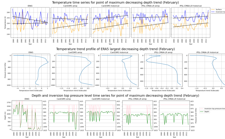
Figure 10: Inversion top and surface time series, trend profile, and depth and inversion top pressure level time series for the point of greatest decreasing depth trend (69°N, 179.5°W in February)
