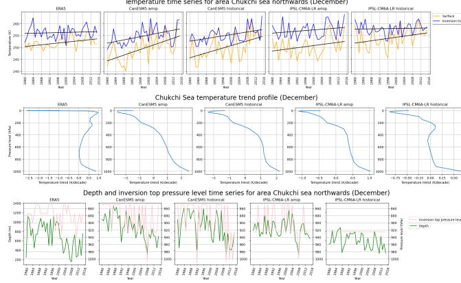
Figure 12: Inversion top and surface time series, trend profile, and depth and inversion top pressure level time series around the Chukchi Sea in December)
