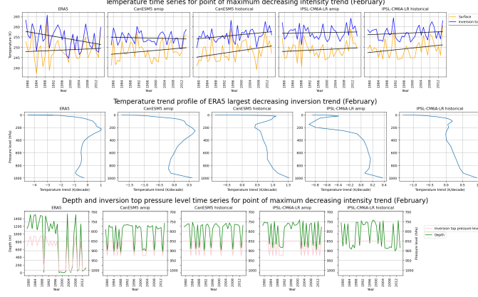
Figure 9: Inversion top and surface time series, trend profile, and depth and inversion top pressure level time series for the point of greatest decreasing intensity trend (67.25°N, 176.25°W in February)
