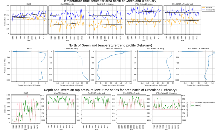
Figure 11: Inversion top and surface time series, trend profile, and depth and inversion top pressure level time series north of Greenland in February)
