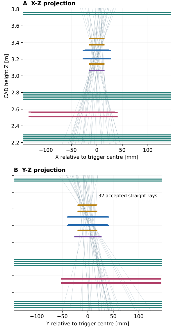
Figure 1: Installed geometry and the accepted-ray aperture. Left: the complete aligned detector model, with passive material shown translucently and a separate enlargement of the central assembly below. CAD stand supports are outside the material model. Right: the previous rate report's 32 accepted straight rays, with its original vector projections stacked for readability. These rays use the earlier offset ECAL; all main-table rates use the aligned layout. Colours identify the same subsystems in both panels. The rays include no scattering or detector response.
