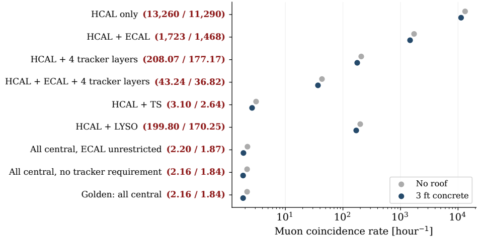
Figure 2: From detector aperture to coincidence rate. (a) The active-layer envelopes, with transverse coordinates measured from the tracker axis and heights in CAD Z . Line thicknesses are enlarged for visibility; the calculation retains the segmented solids. (b) Inclusive selections requiring all ten HCAL layers, on a logarithmic rate axis. “All central” requires all TS, LYSO, ECAL and tracker layers. “ECAL unrestricted” keeps ECAL installed but imposes no ECAL hit requirement: events may hit or miss it, while all other listed hit requirements still apply. “No tracker requirement” similarly leaves tracker hits unrestricted. The same aligned geometry and sea-level spectrum are used for both roof assumptions. Bold red values beside each selection give the rate per hour (no roof / 3 ft concrete).
