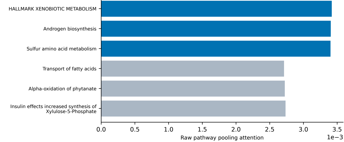
Omics slot 5: Top-3 / Bottom-3
