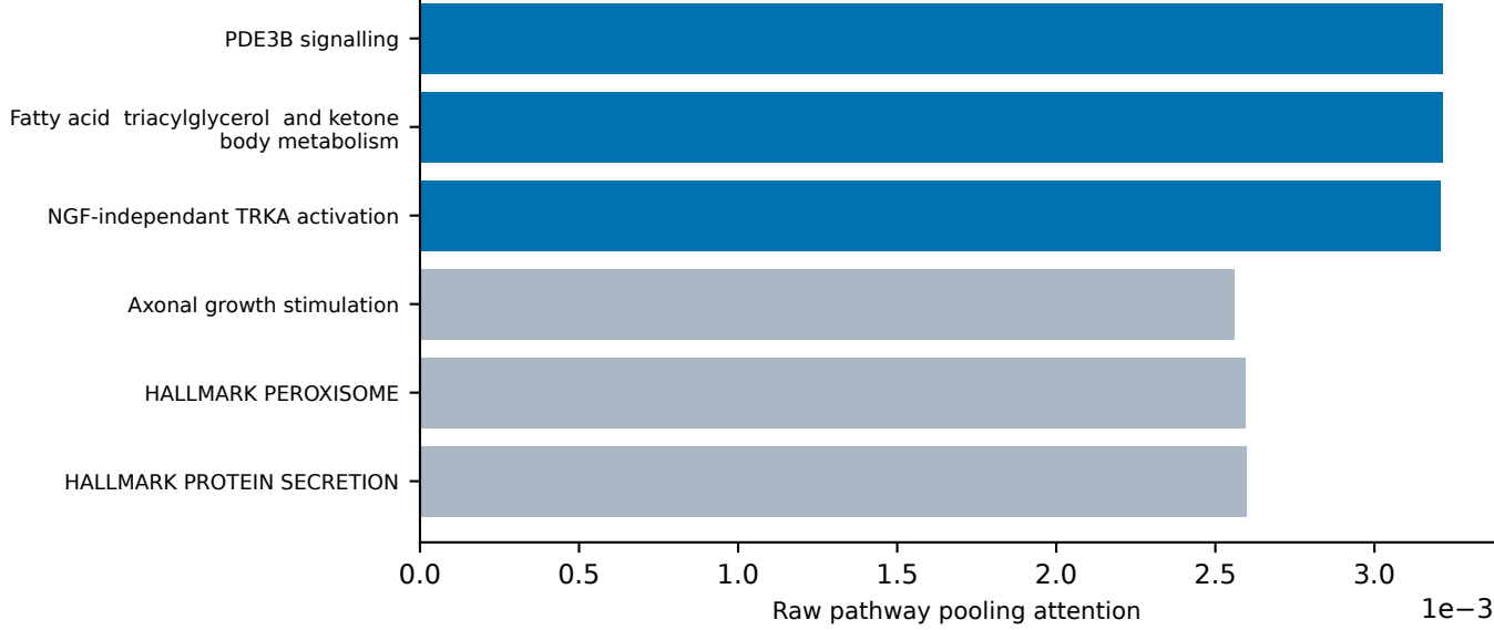
Omics slot 2: Top-3 / Bottom-3
