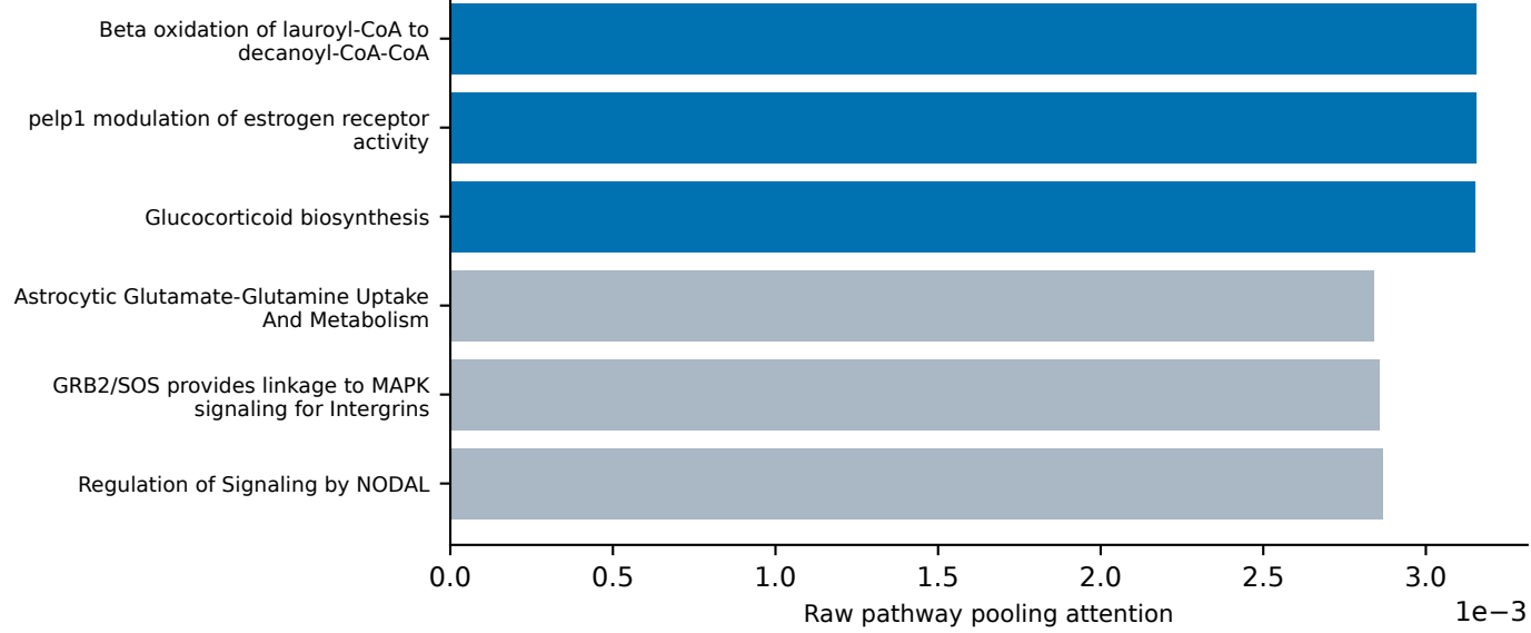
Omics slot 3: Top-3 / Bottom-3
