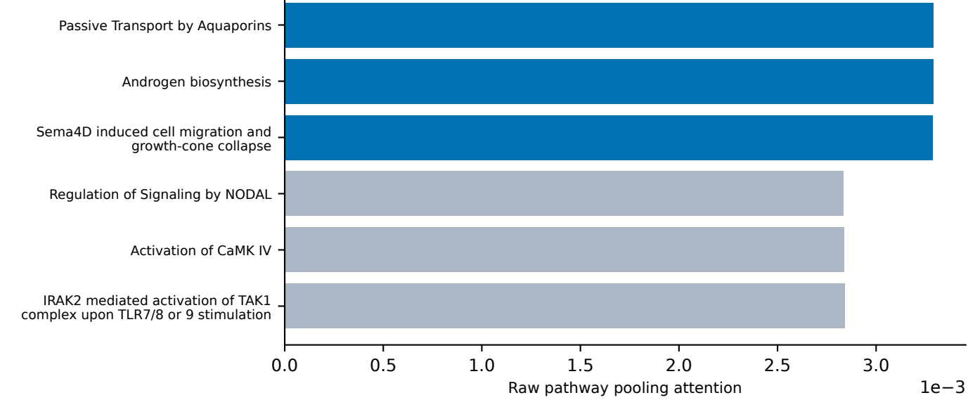
Omics slot 7: Top-3 / Bottom-3
