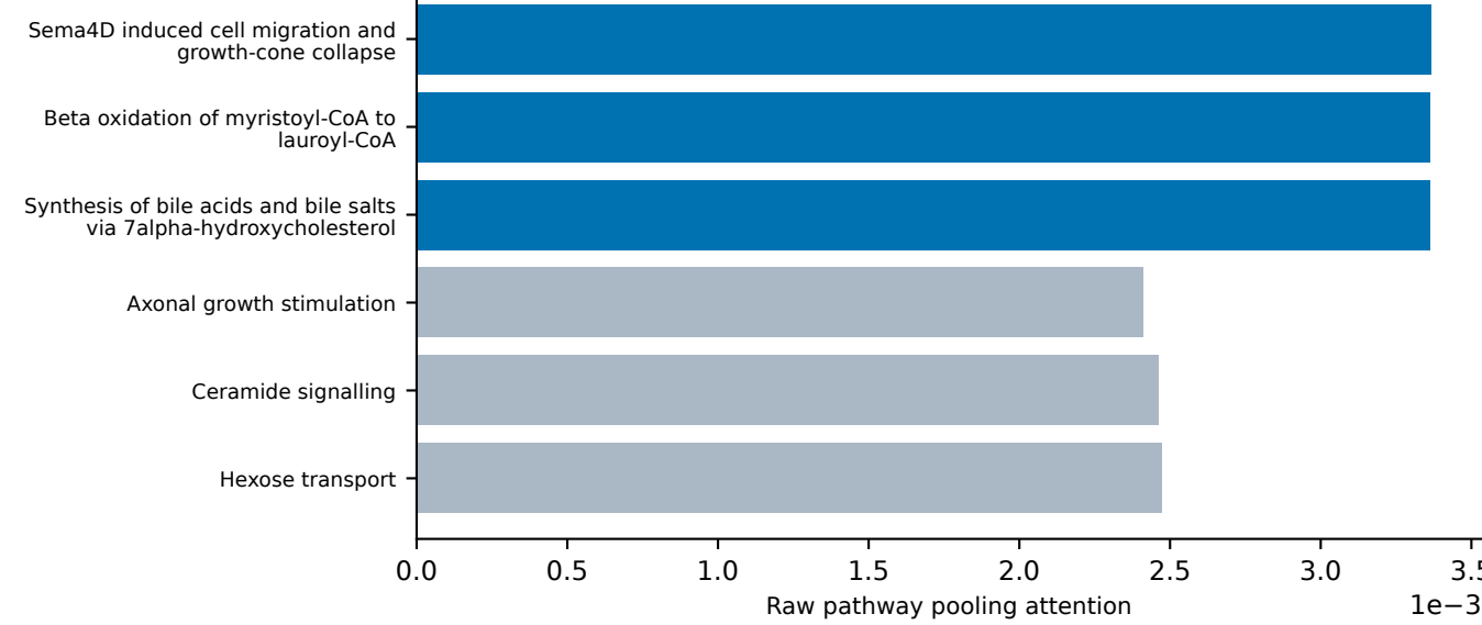
Omics slot 6: Top-3 / Bottom-3
