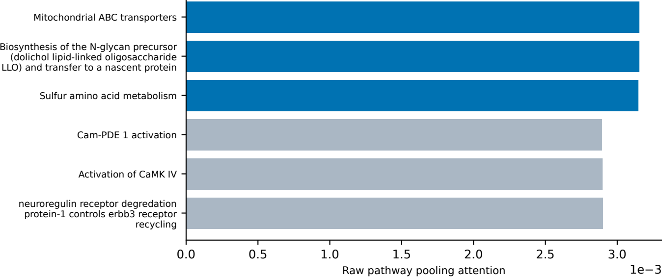
Omics slot 4: Top-3 / Bottom-3
