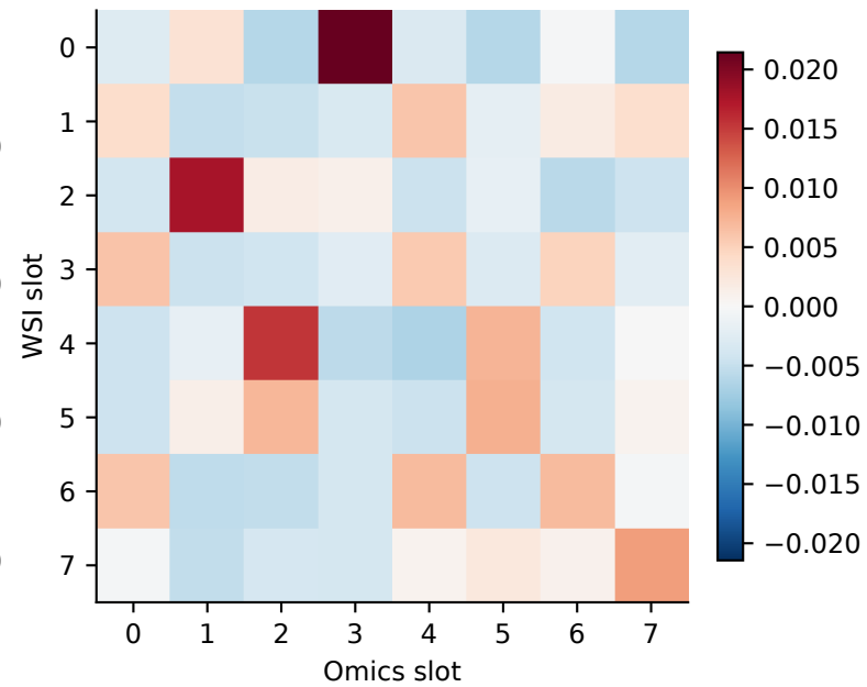
C Learned minus independent
