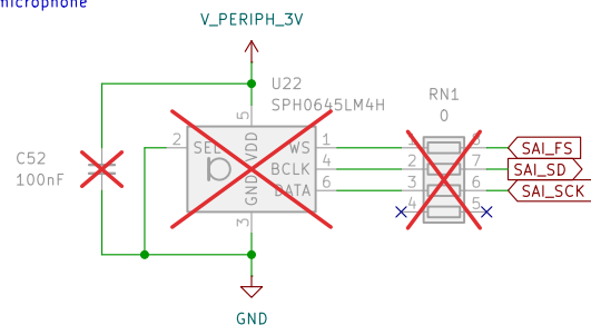
Onboard MEMS microphone
