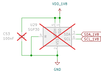
Indoor air quality sensor
