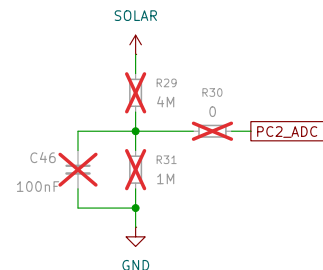
Onboard solar voltage sensing
