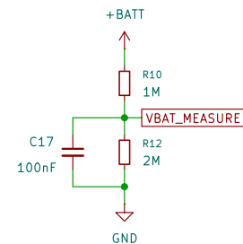
Onboard battery voltage sensing
