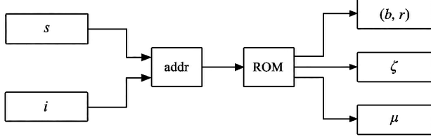
Fig. 8. Address schedule generator.
