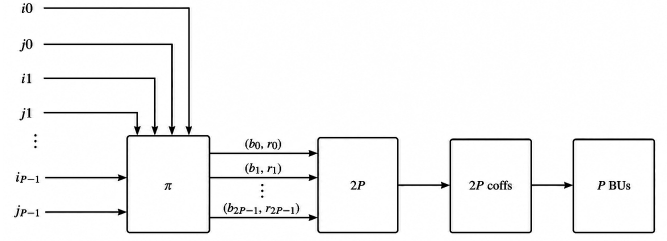
Fig. 9. Conflict-free bank mapping.
