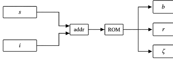
Fig. 7. Schedule ROM interface.
