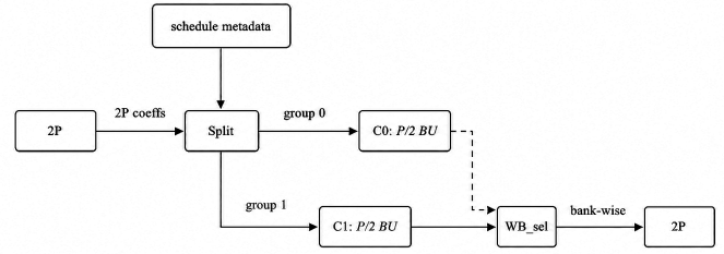
Fig. 9. Conflict-free bank mapping.
