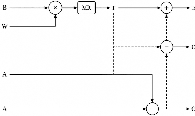
Fig. 3. Cooley-Tukey butterfly.
