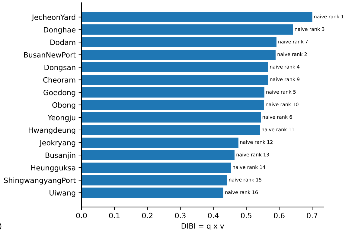
B. Top-15 stations
