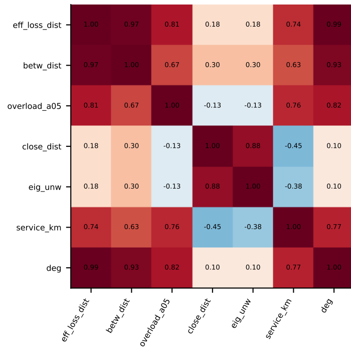
C. Spearman matrix (out-of-scope pool)
