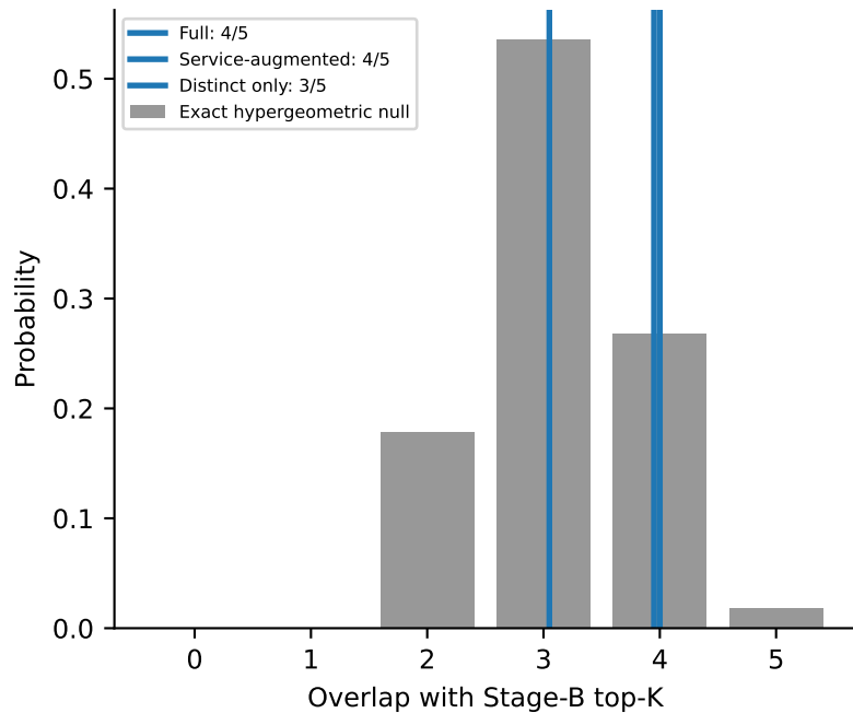
A. Uniform null (exact)
