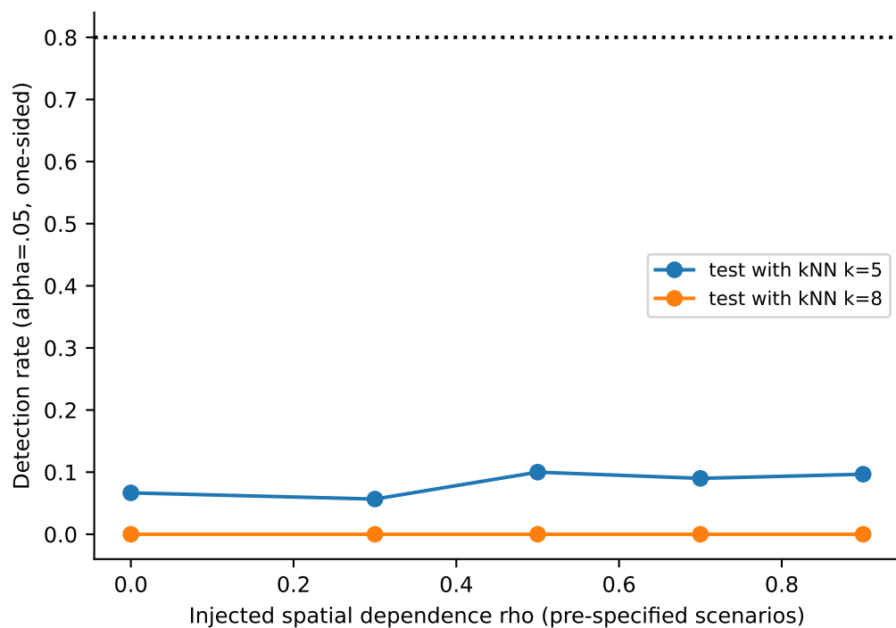
C. Power of Moran's I at N = 8
