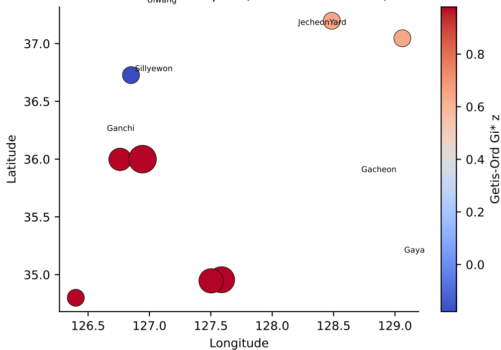
D. Local hot/cold spots (marker size = value)
