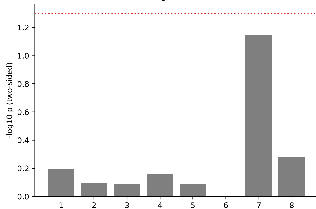
B. No detected global autocorrelation?
