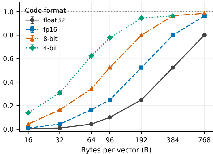
Model A
