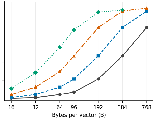
Model B
