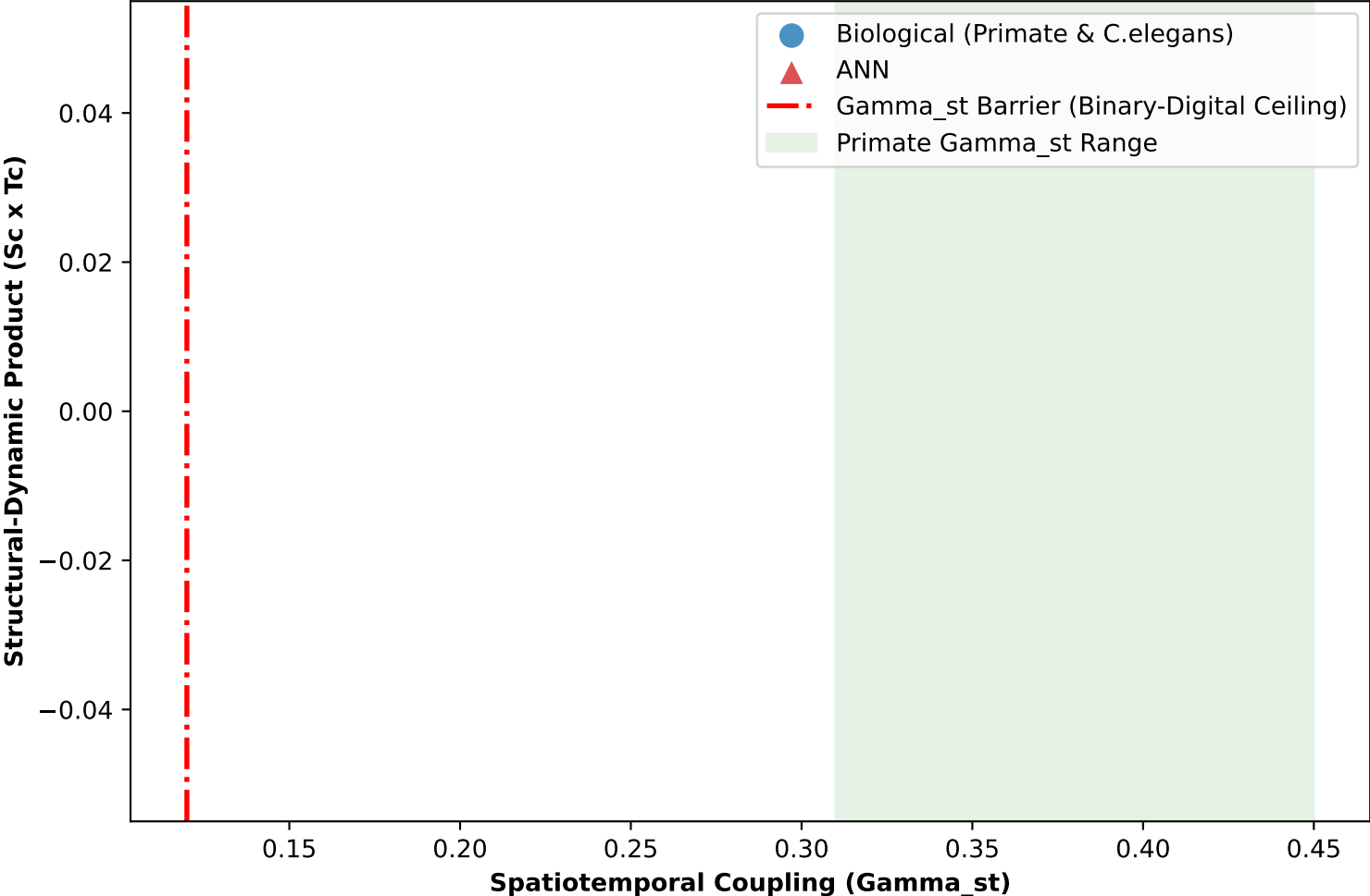
Figure 2. CST Component Space & The Gamma_st Barrier
