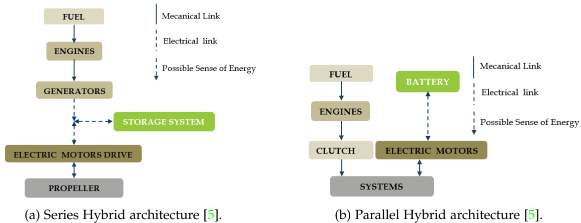
Figure 1.4: Hybridization schemes.
