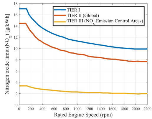
(b) \text{NO}_x limits in terms of engine speed.
