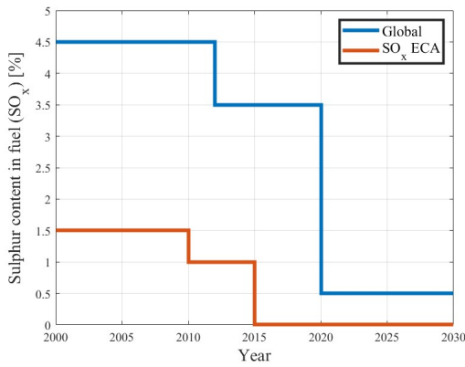
(a) Changes in \text{SO}_x limits over time.
