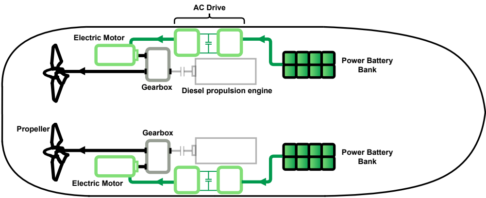
Figure 3.9: Energy flow in PTH mode.
