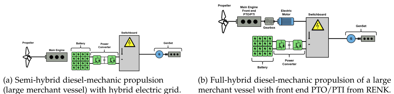
Figure 1.10: Hybridization with diesel propulsion systems.
