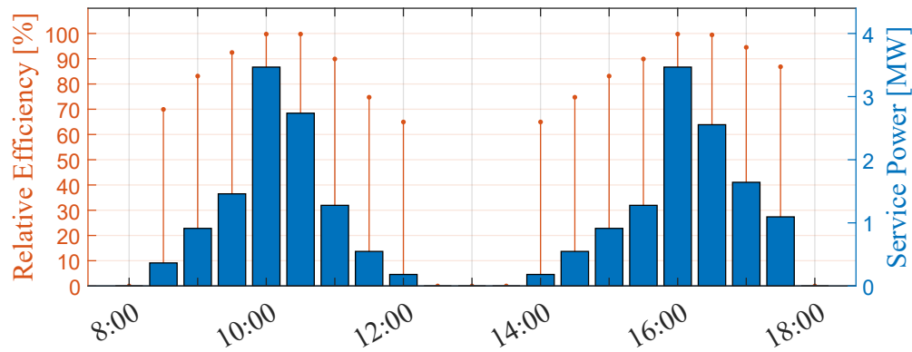
Figure 2.22: Relative efficiency of a convencitonal tugboat: two maneuvers.
