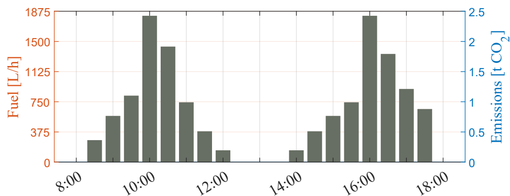
Figure 2.24: Fuel consumption and emissions with respect to the tugboat's operating profile in two maneuvers.
