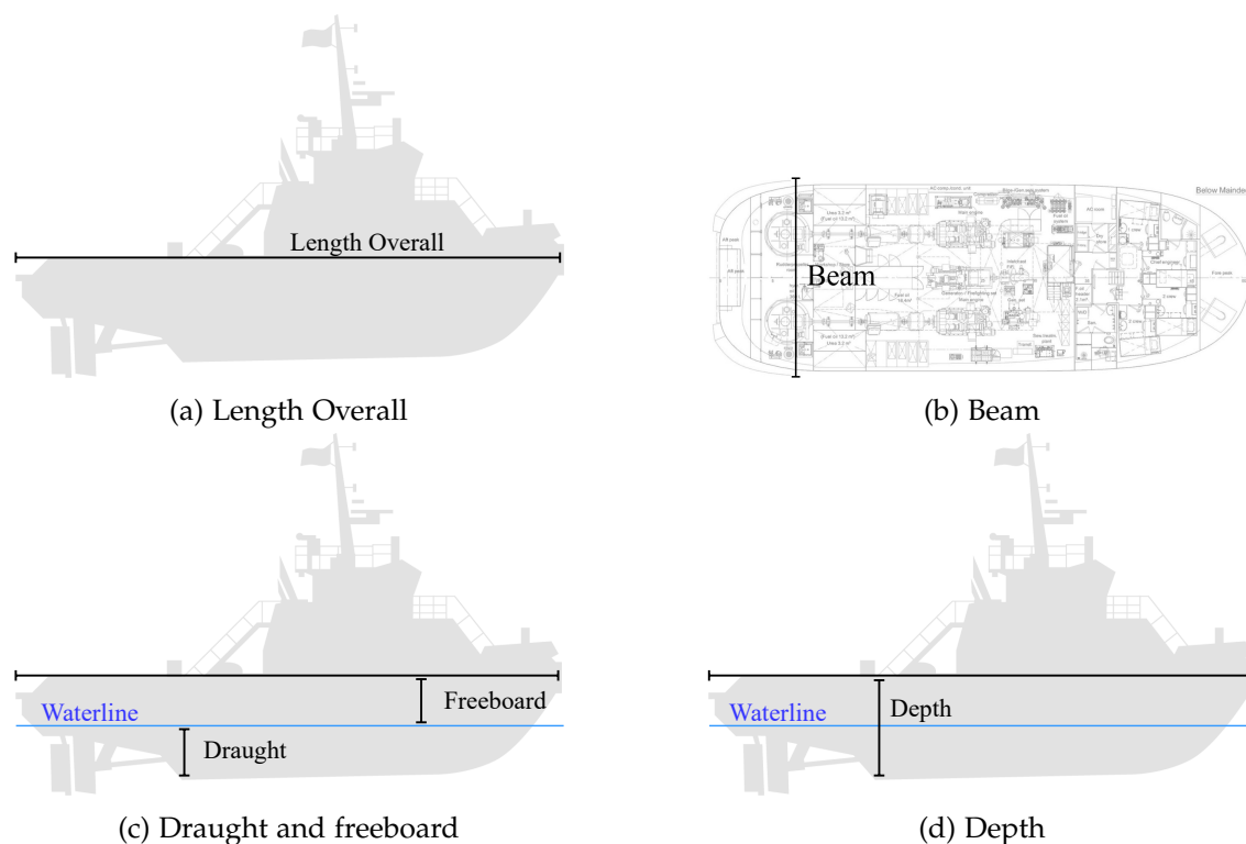
Figure 2.5: Physical dimensions of a tugboat.
