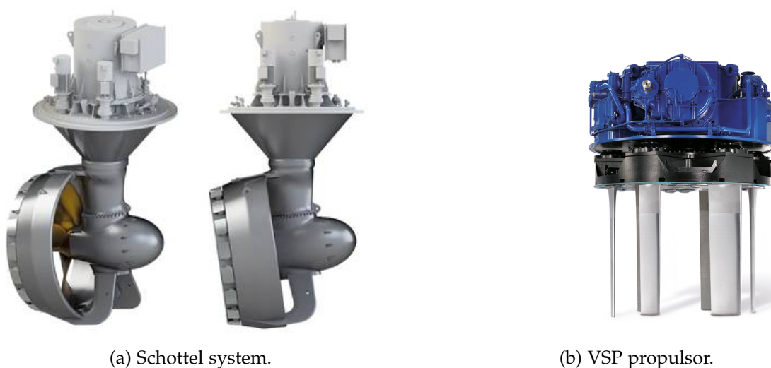
Figure 2.13: Special Propulsors.
