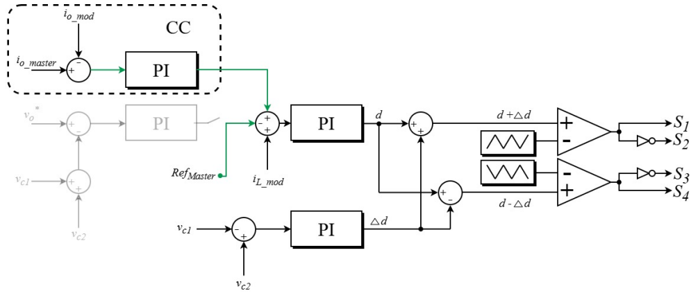
Figure A.8: Proposed Master-Slave control strategy.
