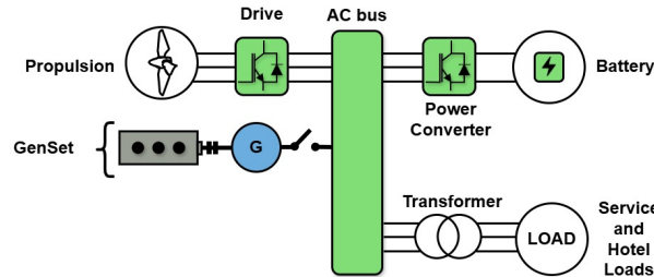
Figure 3.2: Genset inside a hybrid vessel.
