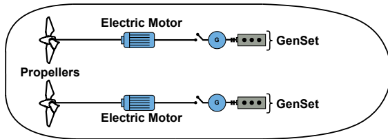
(a) Electric shaft propulsion system.
