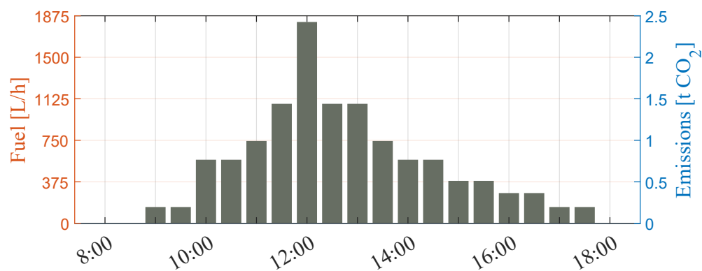
Figure 2.23: Fuel consumption and emissions with respect to the tugboat's operating profile during a maneuver.
