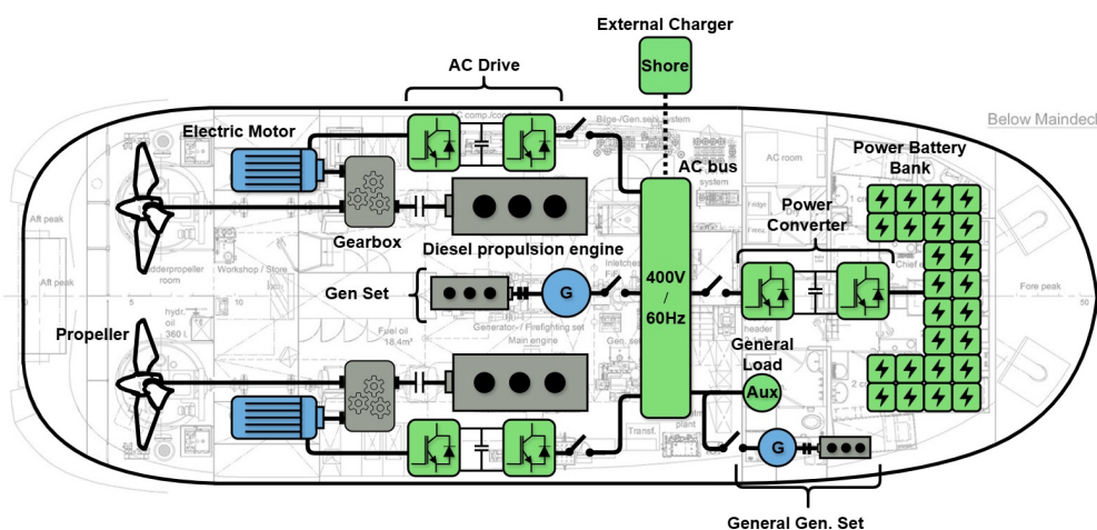
Figure 3.14: General Scheme
