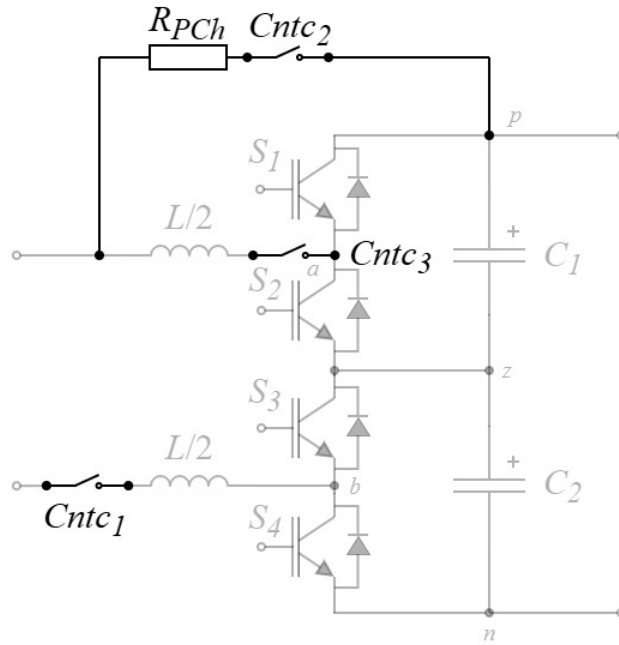
Figure A.7: Implementation of contactors in TLBBC for capacitor precharging process.
