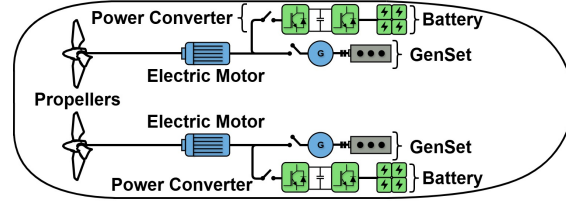
(b) Electric shaft with electric energy storage system.
