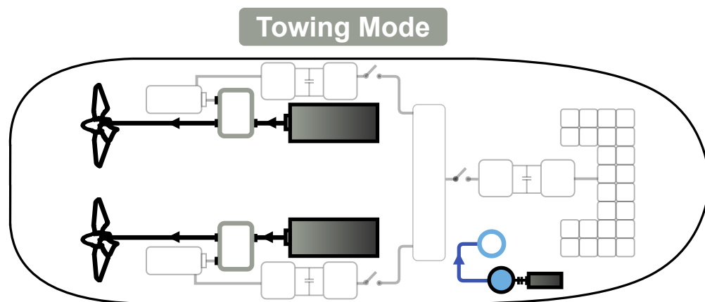
Figure 3.15: Towing Mode
