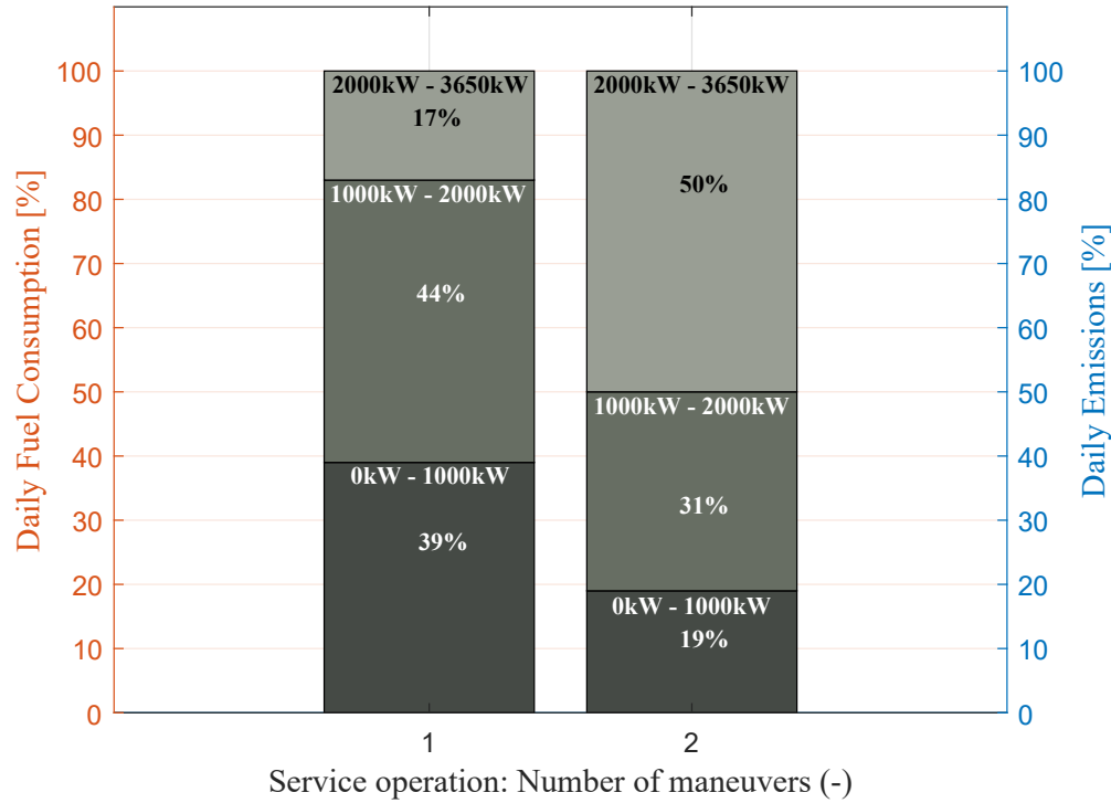
Figure 2.25: Percentage of emissions per day based on power ranges.
