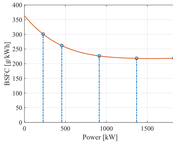
Figure 2.20: Brake-specific fuel consumption of a diesel engine model Cat 3516 B.
