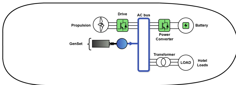
Figure 3.10: Scheme of AC Link into the tugboat.
