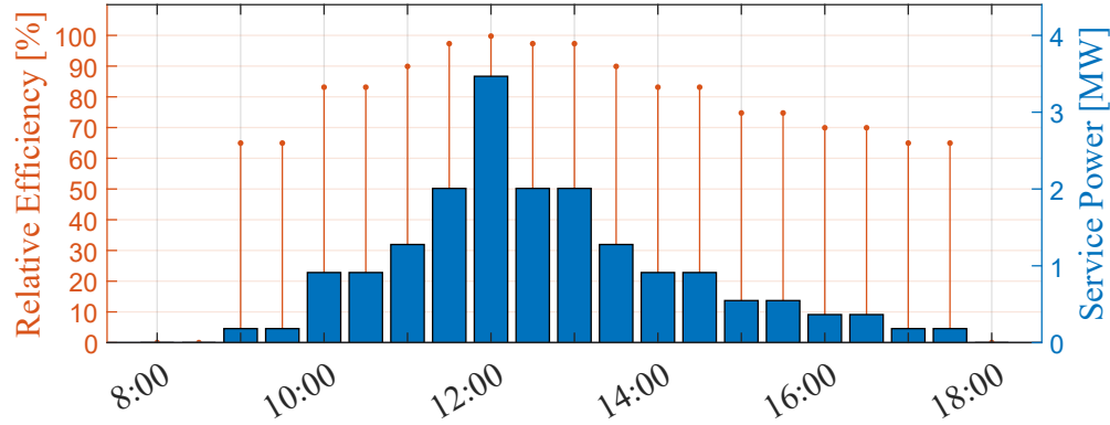
Figure 2.21: Relative efficiency of a convencitonal tugboat: one maneuver.
