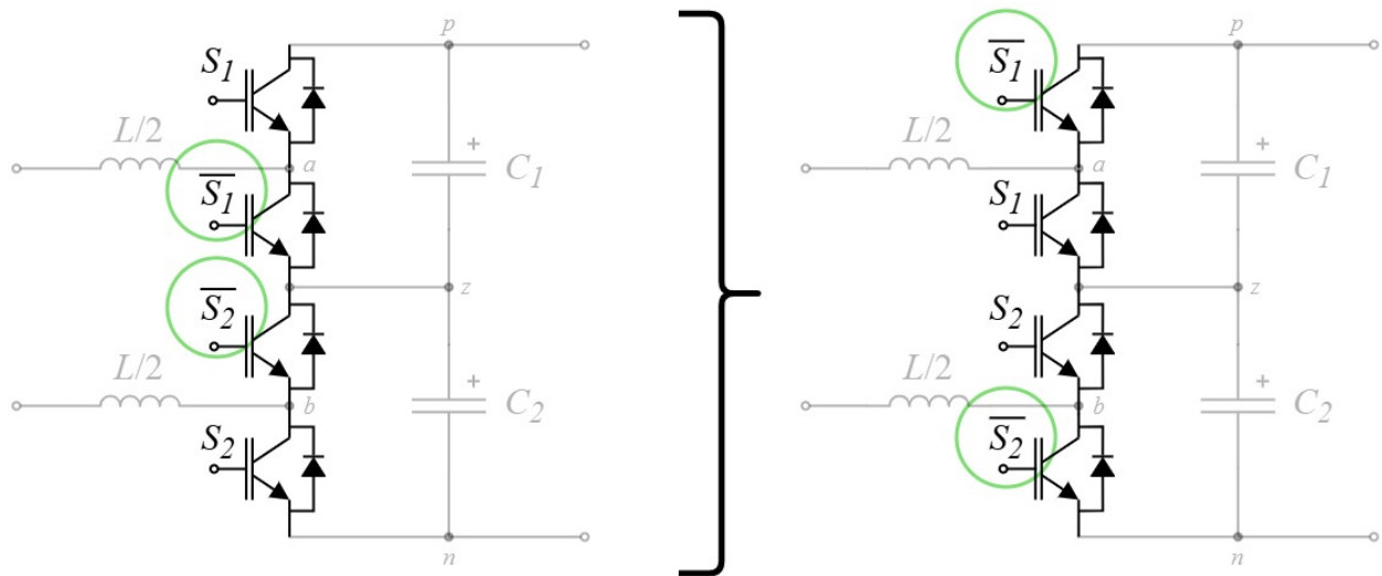
Figure 7.1: Changes in the selection of the firing logic for the upper and lower phases of the TLBBC converter.
