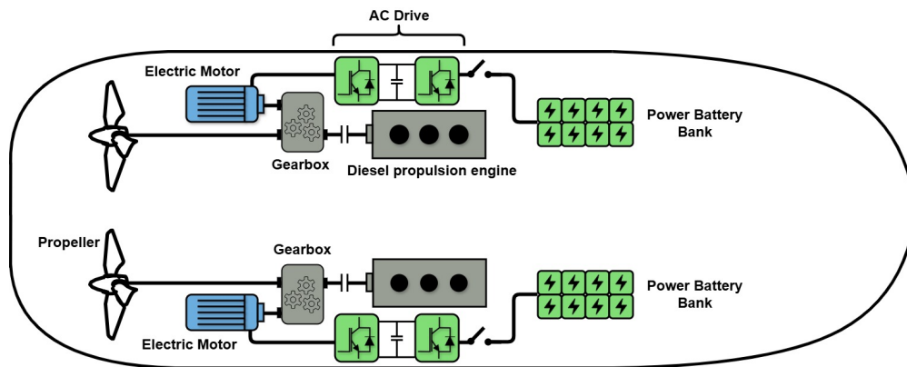
Figure 3.6: Scheme of a parallel hybrid propulsion system.
