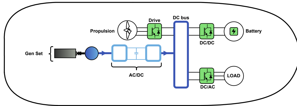
Figure 3.11: Scheme of DC Link into the tugboat.
