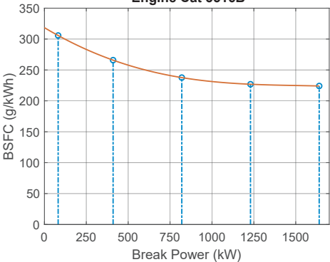
Engine Cat 3516B
