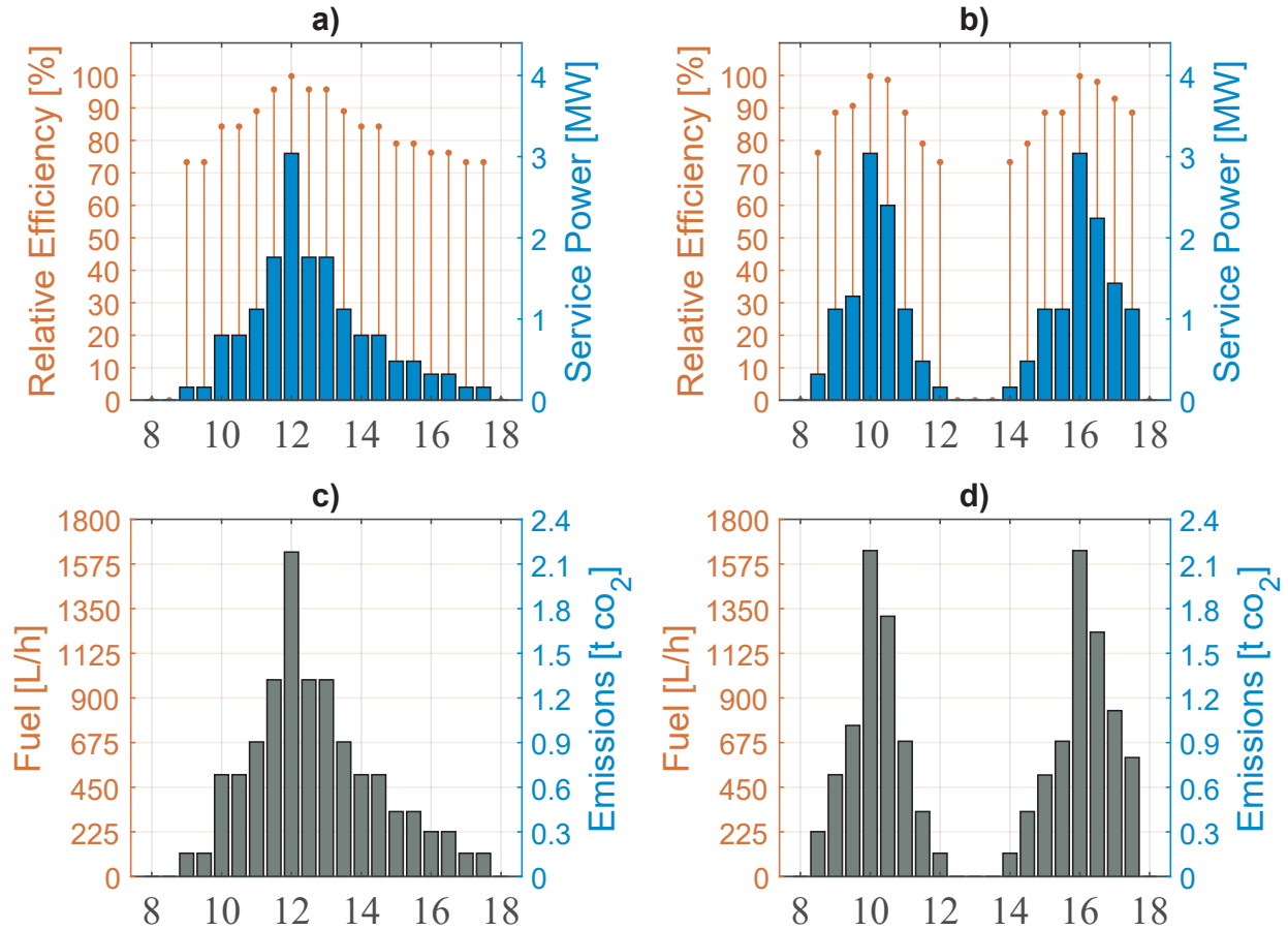
Figure 2.3: Load profile of a tugboat operating in a Chilean harbor: a) One service manoeuvre, b) Two service manoeuvres, c) Fuel consumption/emissions generated for a service maneuver, d) Fuel consumption/emissions generated for two service maneuvers.
