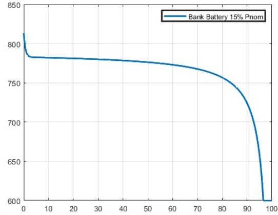
Figure 5.4: discharge curve.
