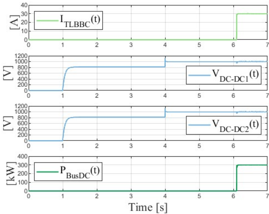
Figure 5.6: BusDC.
