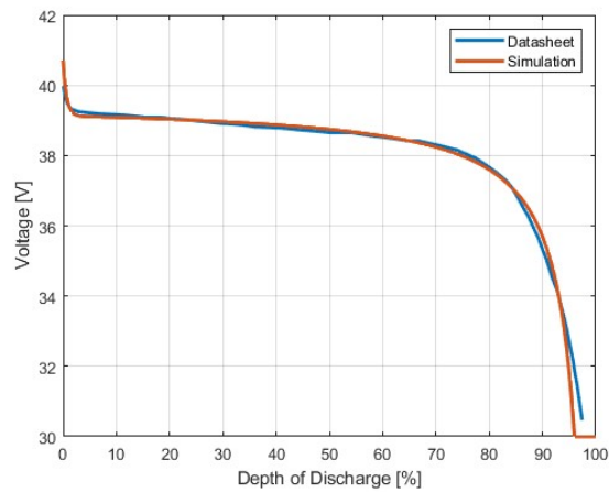
Figure 5.3: discharge curve.
