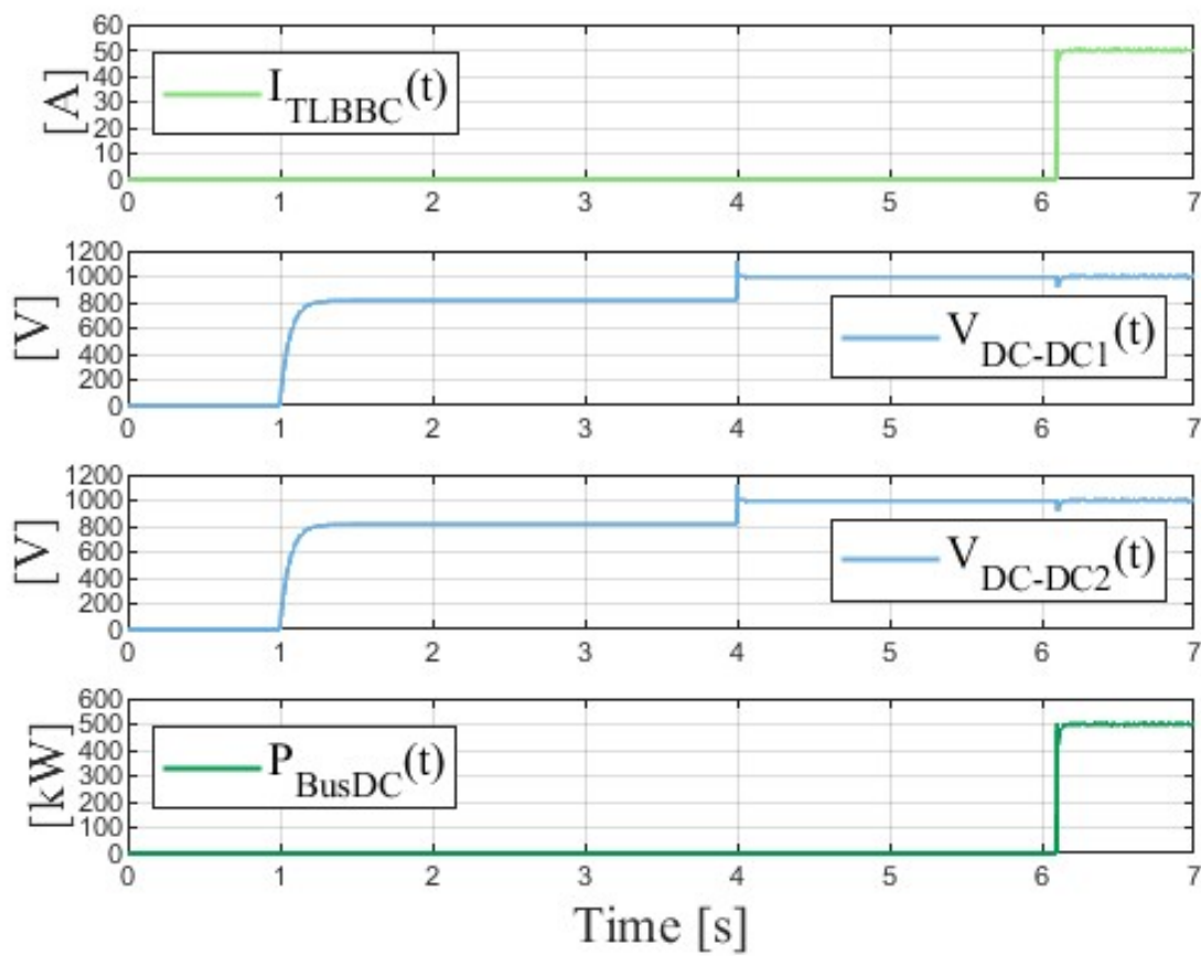
Figure 5.7: BusDC.
