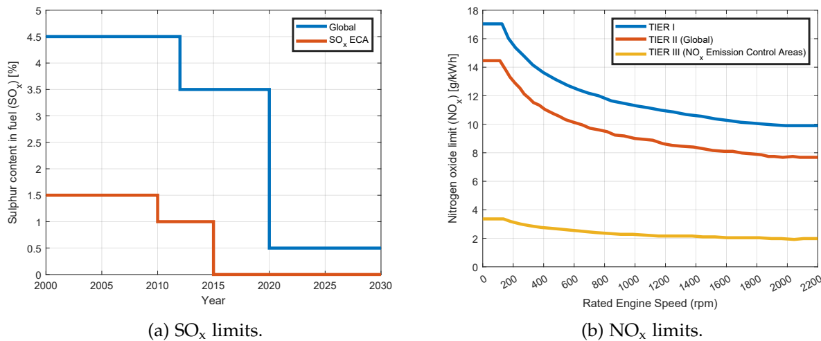
Figure 1.3: The MARPOL Annex VI emission limits for global and Emission Controlled Areas (ECAs perspective).
