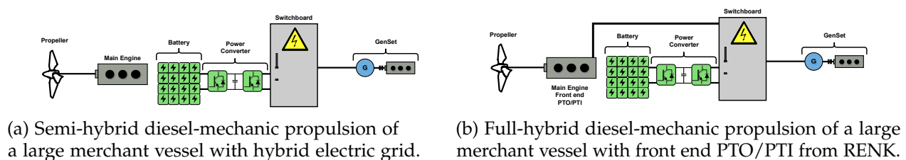
Figure 1.10: Semi-hybridization.
