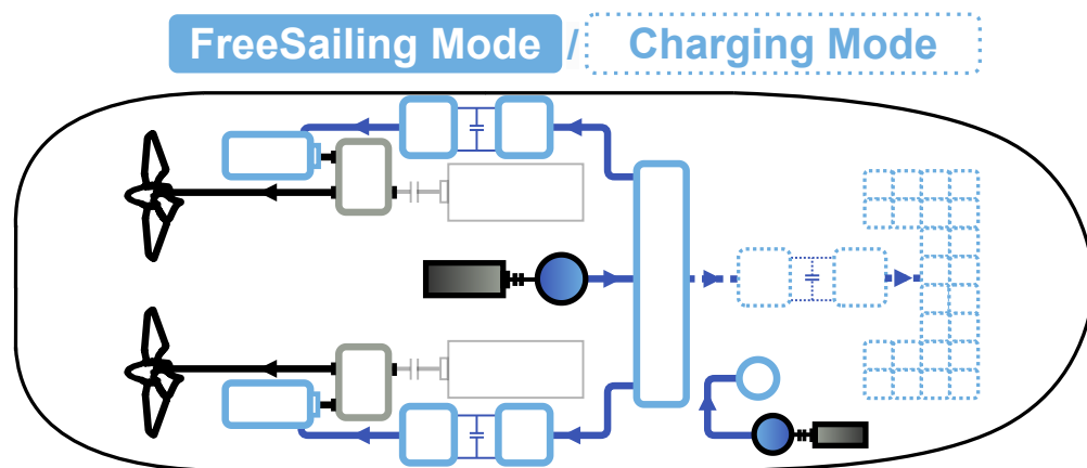
Figure 3.16: FreeSailingMode
