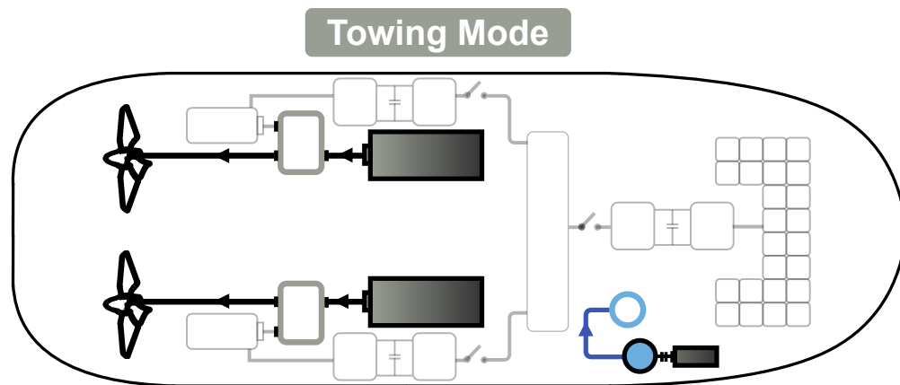
Figure 3.15: Towing Mode
