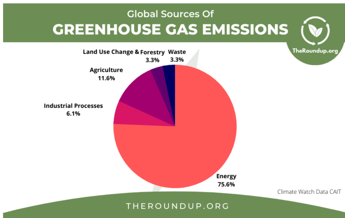
Figure 1.1: Global sources of greenhouse gas emissions [1].
