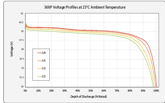
(b) Electrical profile battery cell.
