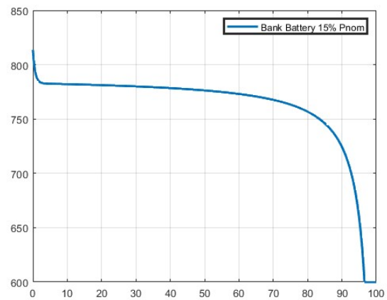
Figure 5.5: discharge curve.
