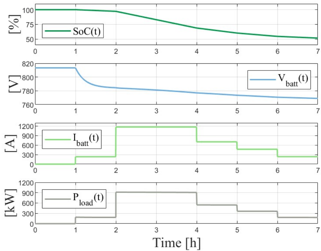
Figure 5.9: discharge curve.
