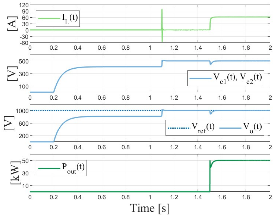
Figure 5.14: BusDC.
