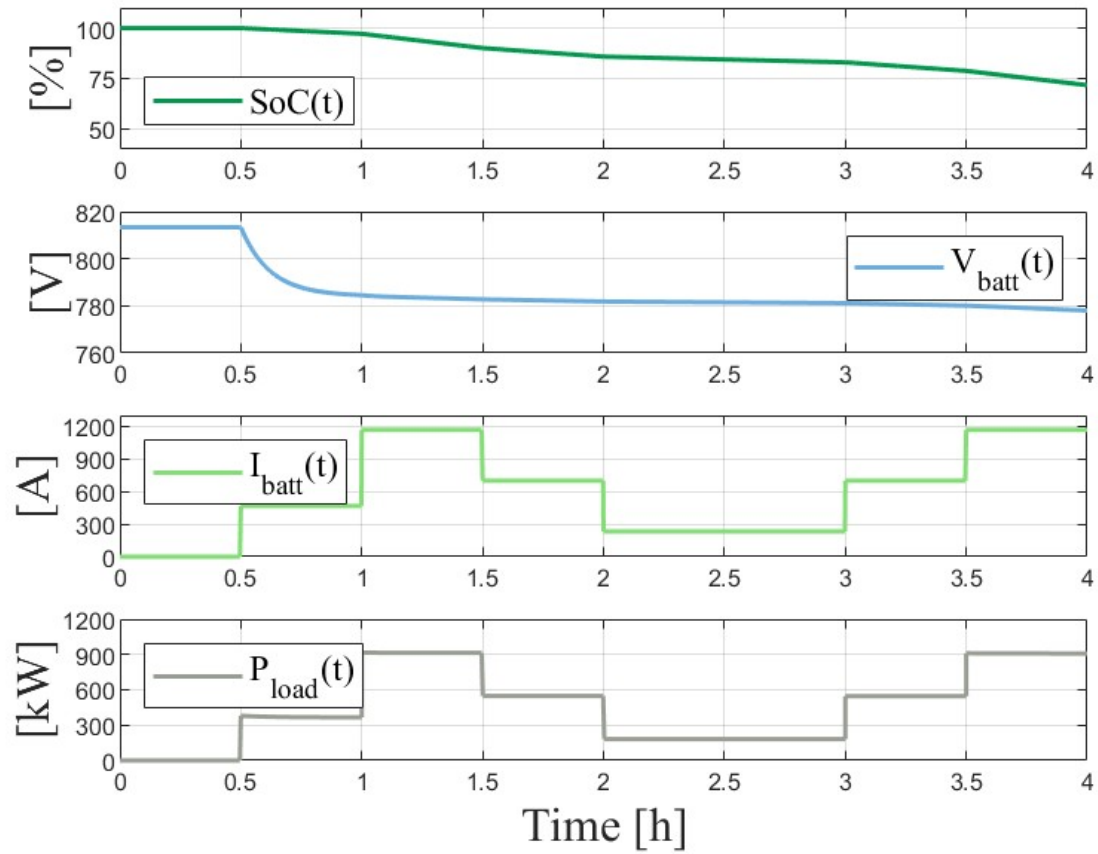
Figure 5.10: discharge curve.
