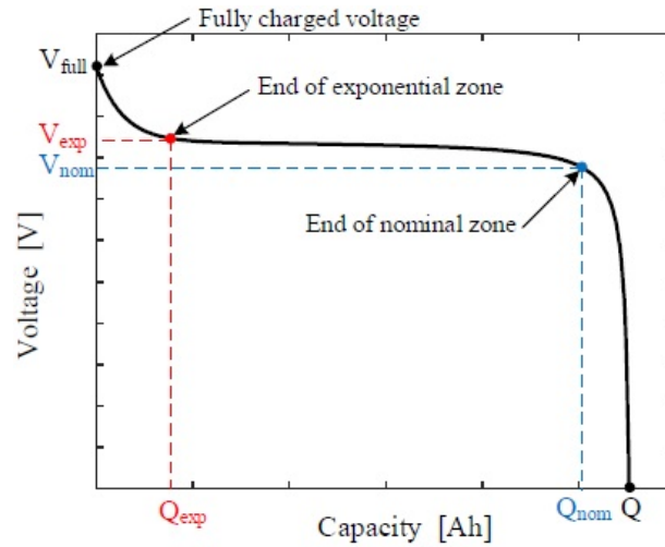
Figure 5.2: discharge curve.
