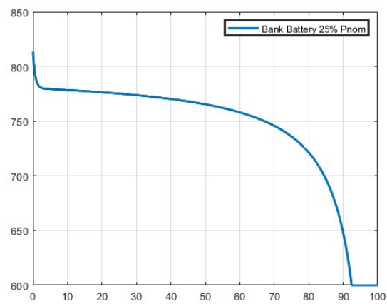
Figure 5.8: discharge curve.
