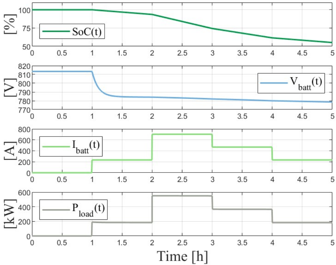
Figure 5.6: discharge curve.
