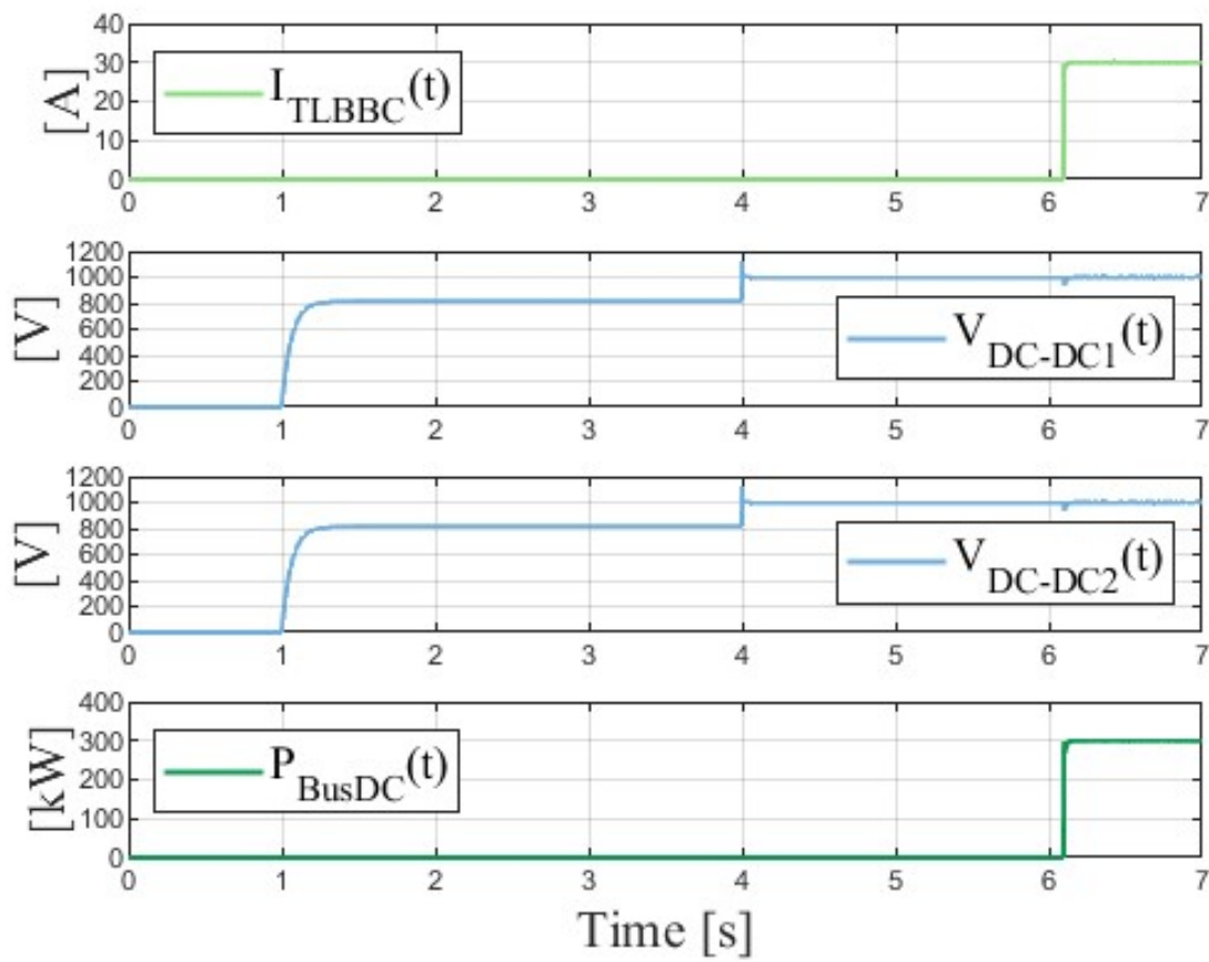
Figure 5.13: BusDC.
