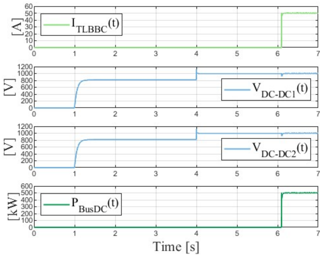
Figure 5.15: BusDC.
