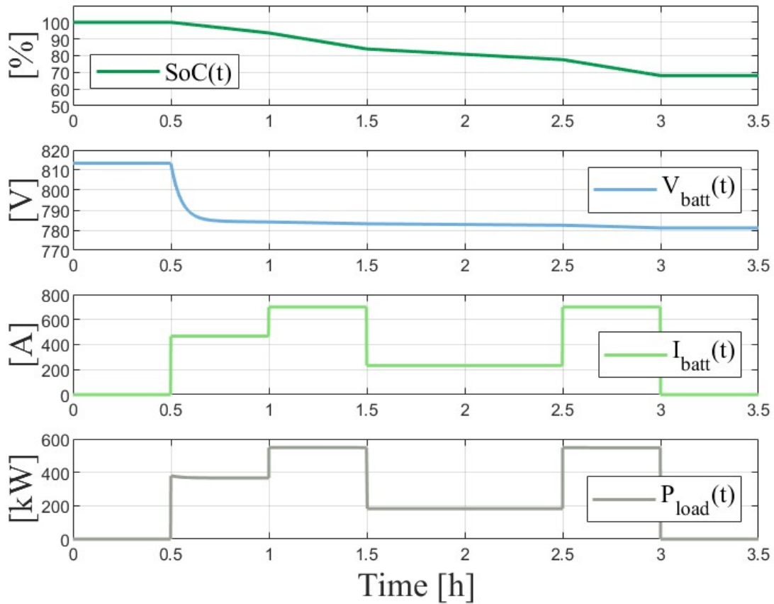
Figure 5.7: discharge curve.
