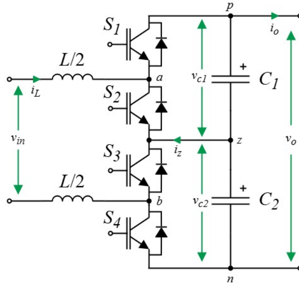
Figure 6.1: BusDC.
