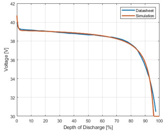
Figure 5.3: discharge curve.
