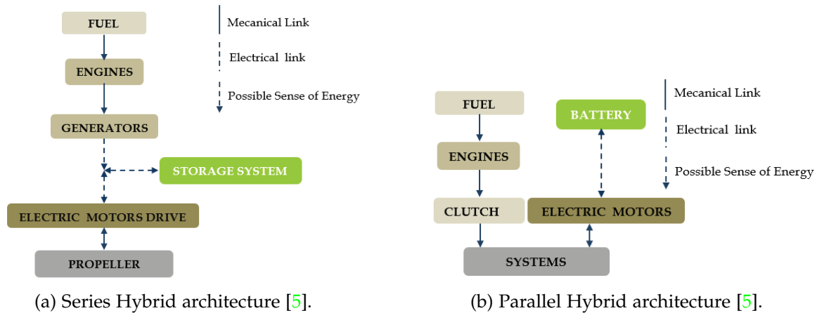
Figure 1.4: Hybridization options.
