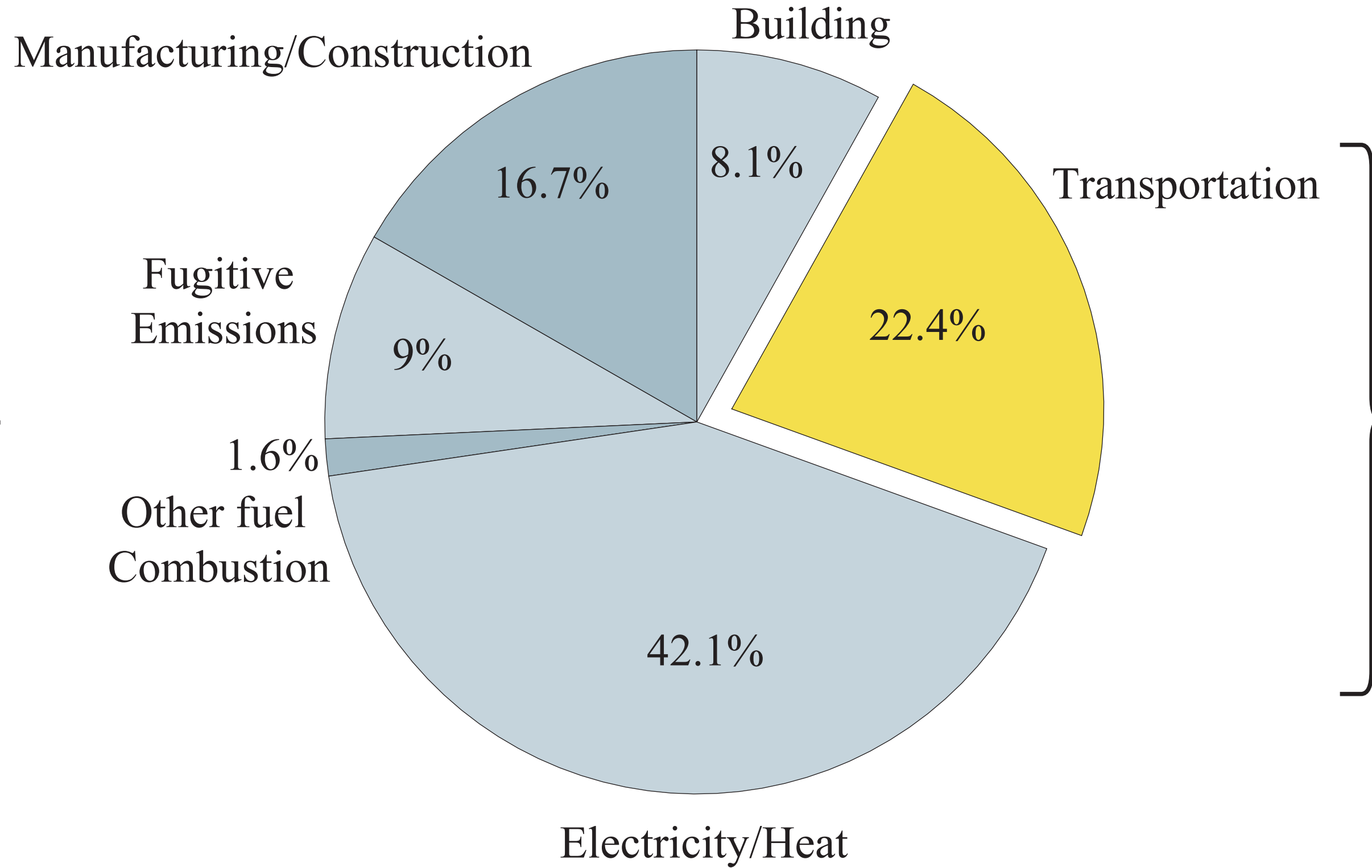
GHG emissions from Energy Sector
