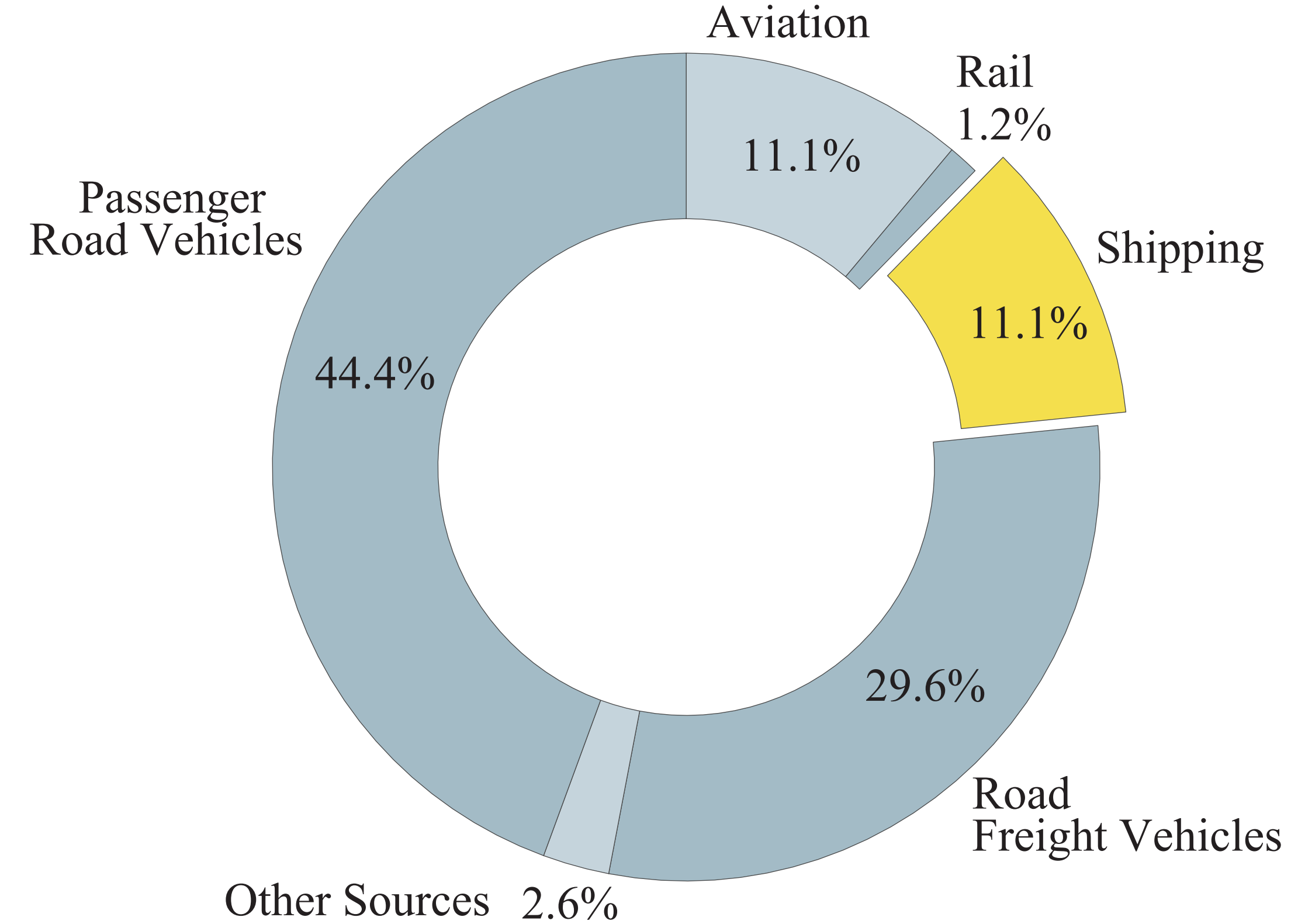
GHG emissions from Transport Sector
