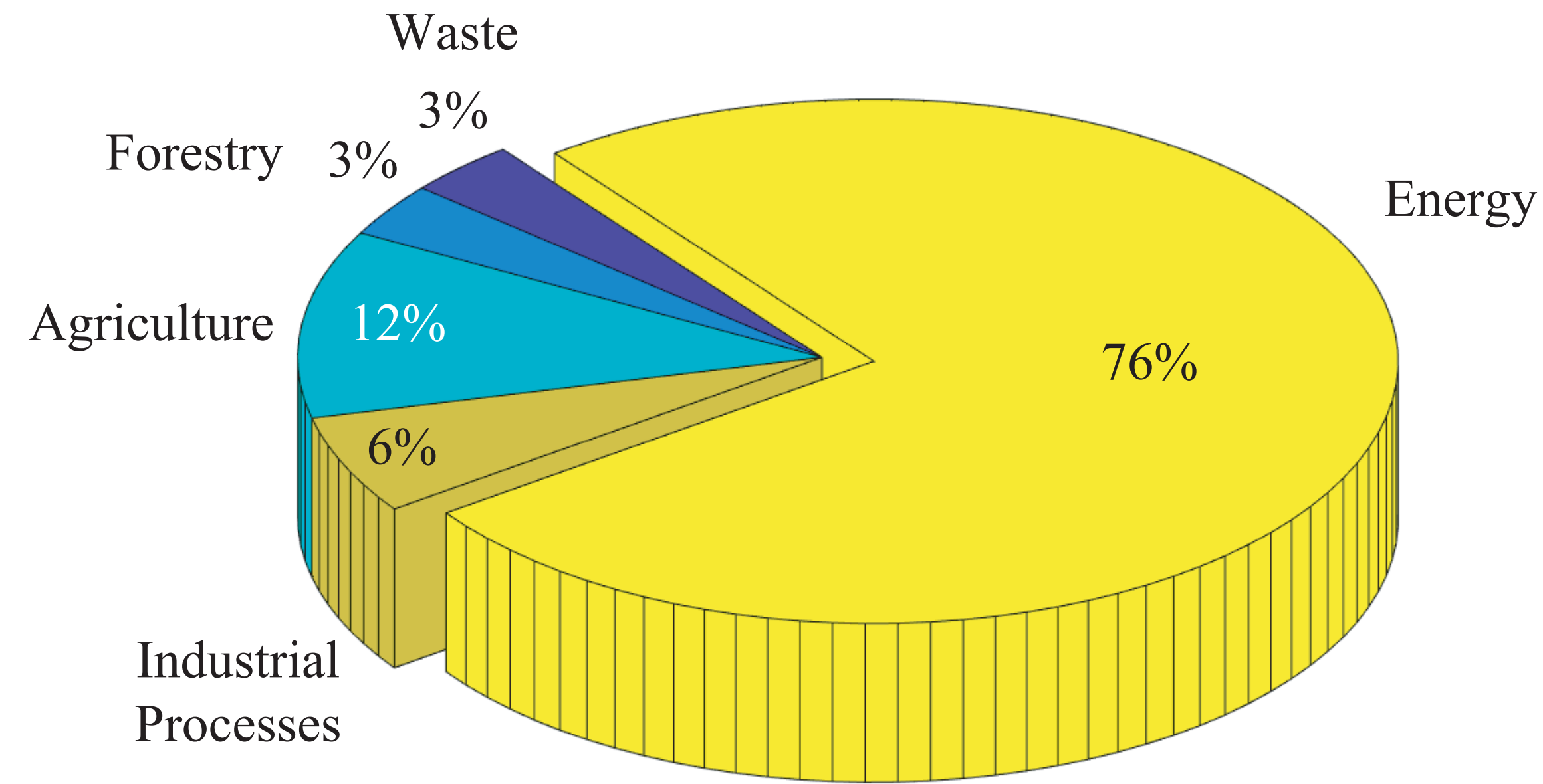
Global sources of Greenhouse Gas Emissions (GHG)
