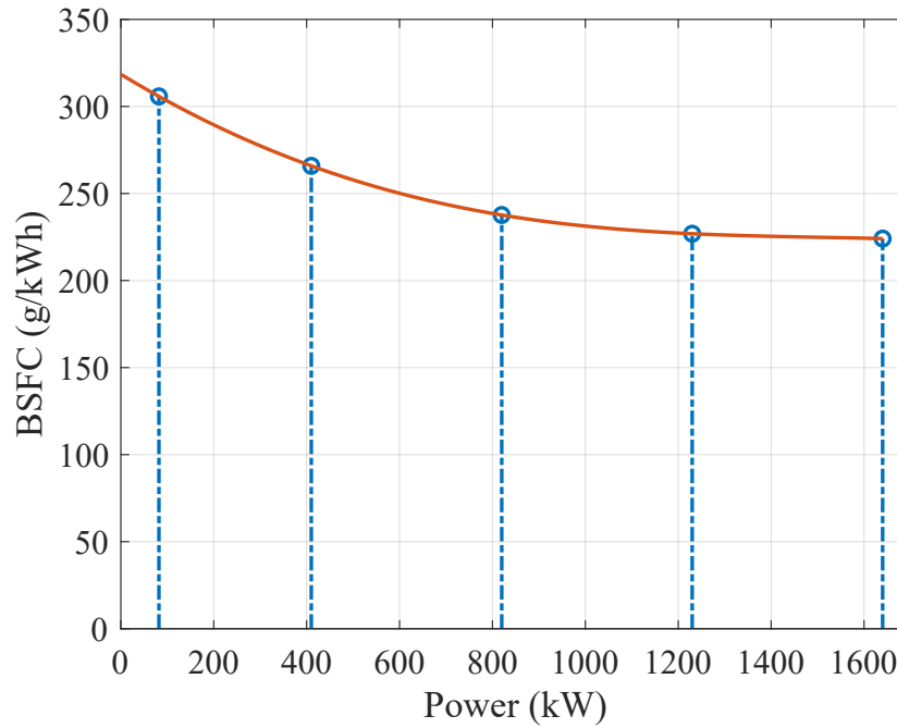
Figure 2.19: Brake-specific fuel consumption of a diesel engine model Cat 3516 B.
