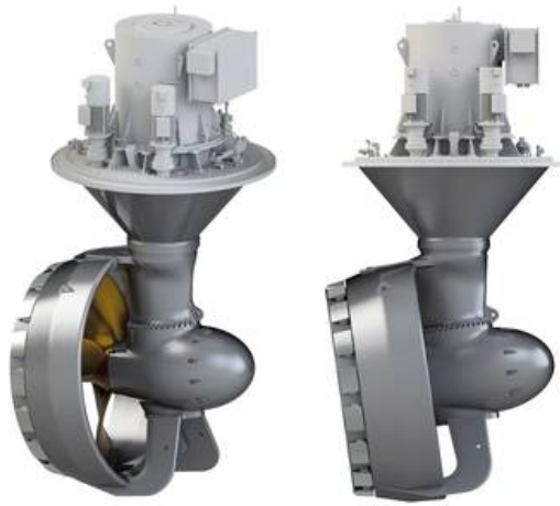
Figure 2.11: Schottel system.
