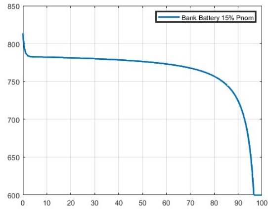
Figure 5.4: discharge curve.
