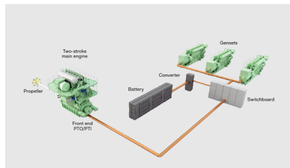
(b) Full-hybrid diesel-mechanic propulsion of a large merchant vessel with front end PTO/PTI from RENK.
