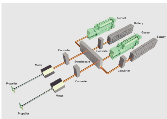
(a) Full-hybrid diesel-electric propulsion with batteries in a hybrid system
