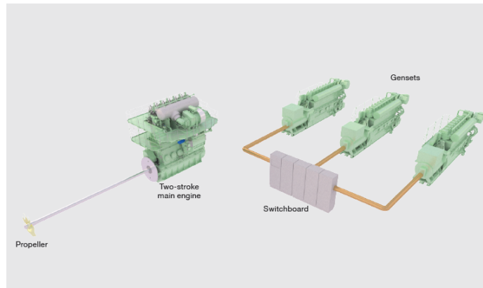
Figure 1.6: Traditional diesel-mechanic propulsion of a large merchant vessel.
