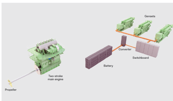
(a) Semi-hybrid diesel-mechanic propulsion of a large merchant vessel with hybrid electric grid
