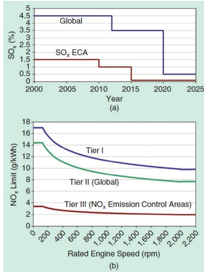
Figure 1.3: The MARPOL Annex VI emission limits for global and Emission Controlled Areas (ECAs perspective) (a) SO x and (b) NO x . (Source: DieselNet) -- > PLOT MATLAB
