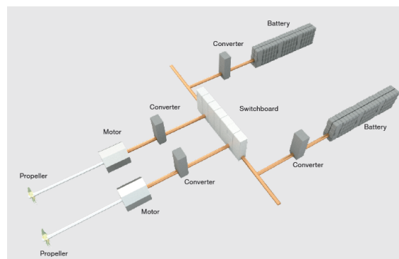
(b) Pure battery-electric propulsion.
