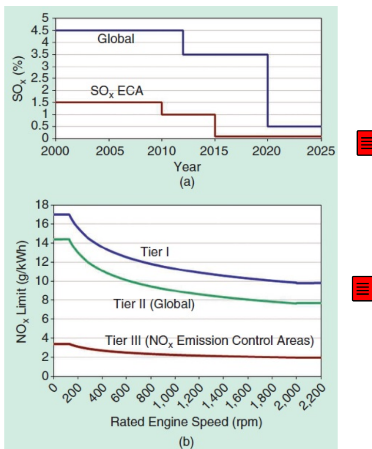
Figure 1.3: The MARPOL Annex VI emission limits for global and Emission Controlled Areas (ECAs perspective) (a) SO x and (b) NO x . (Source: DieselNet)
