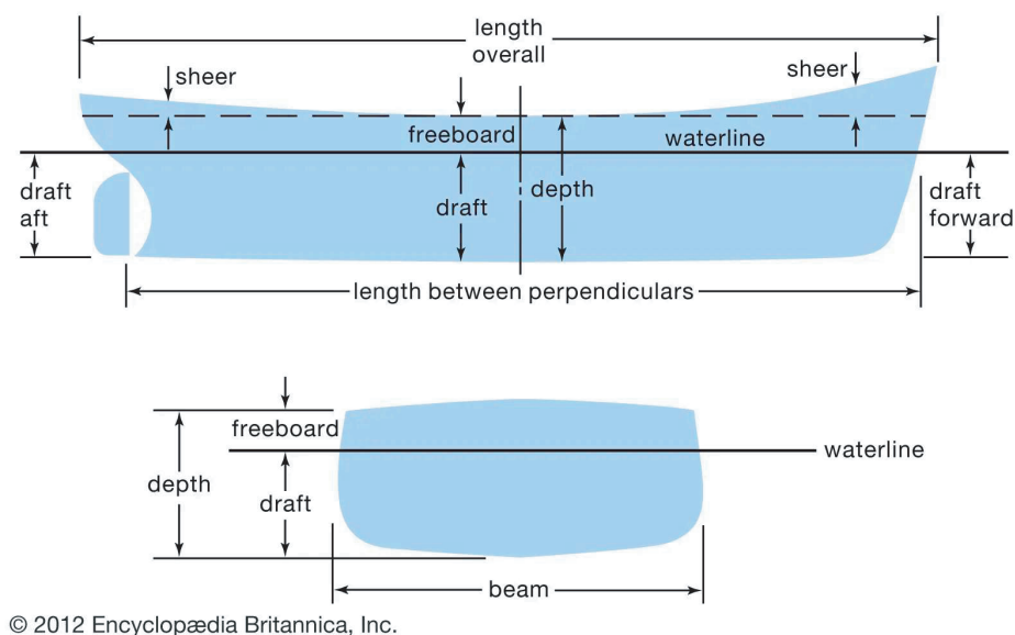
Figure 2.5: dimensions Tug
