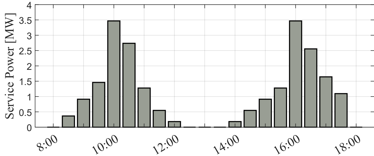
Figure 2.20: Operational profile: Two maneuvers.
