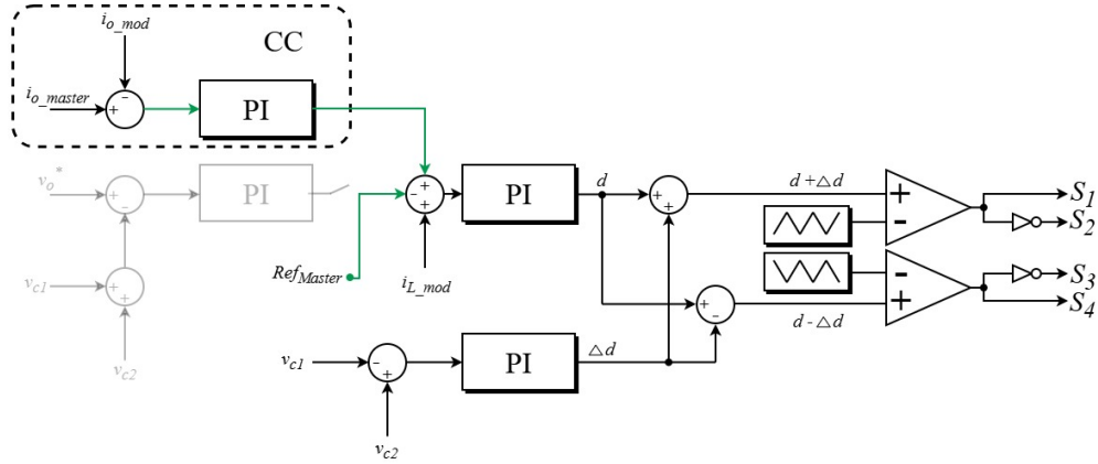
Figure A.8: Proposed Master-Slave control strategy.
