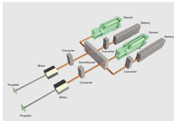
Figure 1.11: Full-hybrid diesel-electric propulsion with batteries in a hybrid system
