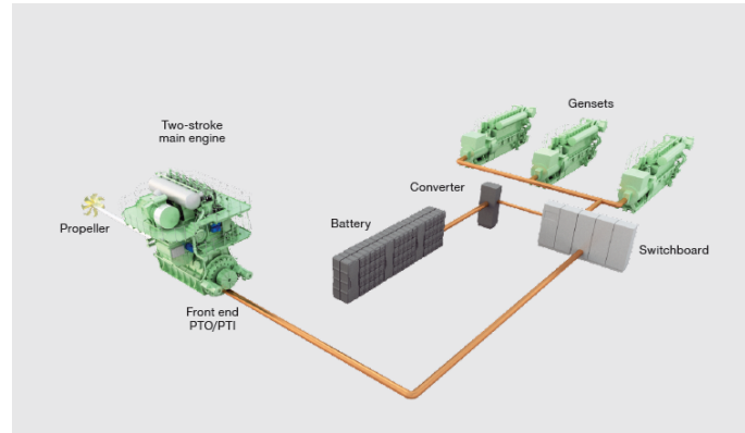
Figure 1.10: Full-hybrid diesel-mechanic propulsion of a large merchant vessel with front end PTO/PTI from RENK.
