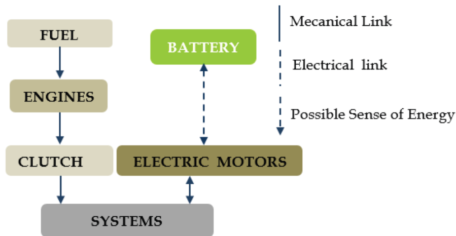
Figure 1.6: Parallel Hybrid architecture.
