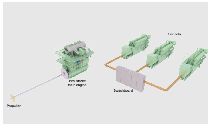
Figure 1.8: Traditional diesel-mechanic propulsion of a large merchant vessel.
