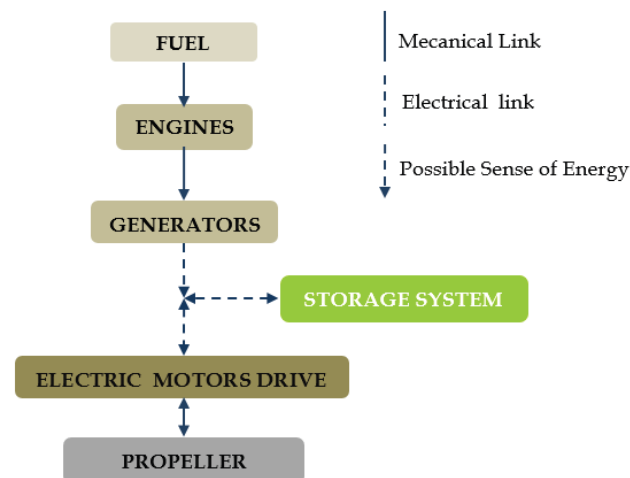
Figure 1.5: Series Hybrid architecture.
