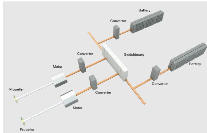
Figure 1.7: Pure battery-electric propulsion.
