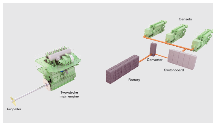
Figure 1.9: Semi-hybrid diesel-mechanic propulsion of a large merchant vessel with hybrid electric grid
