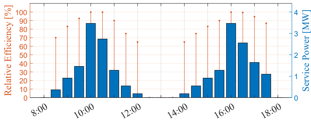
Figure 2.23: Relative efficiency of a conventional tugboat: two maneuvers.
