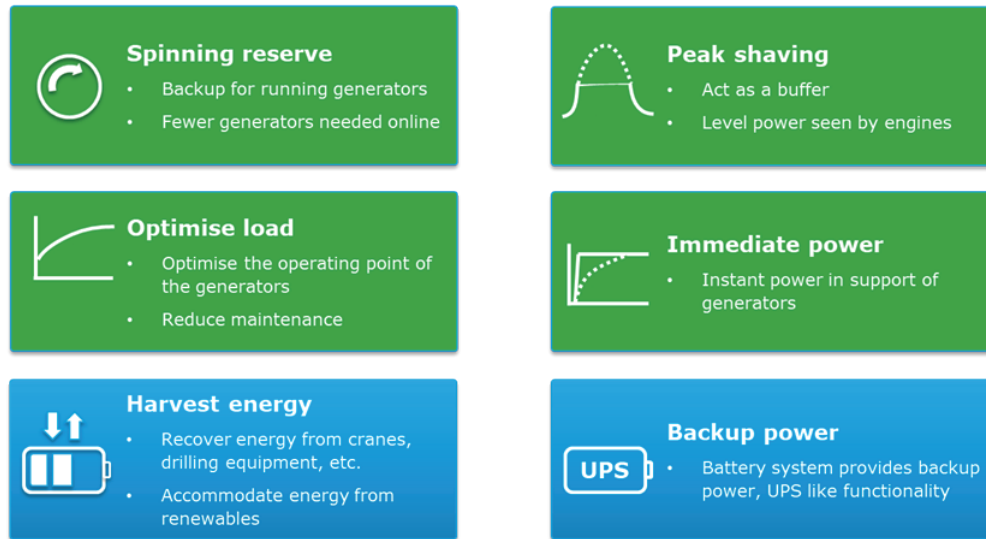
Figure 1.6: Functional roles of battery systems onboard ships [19].
